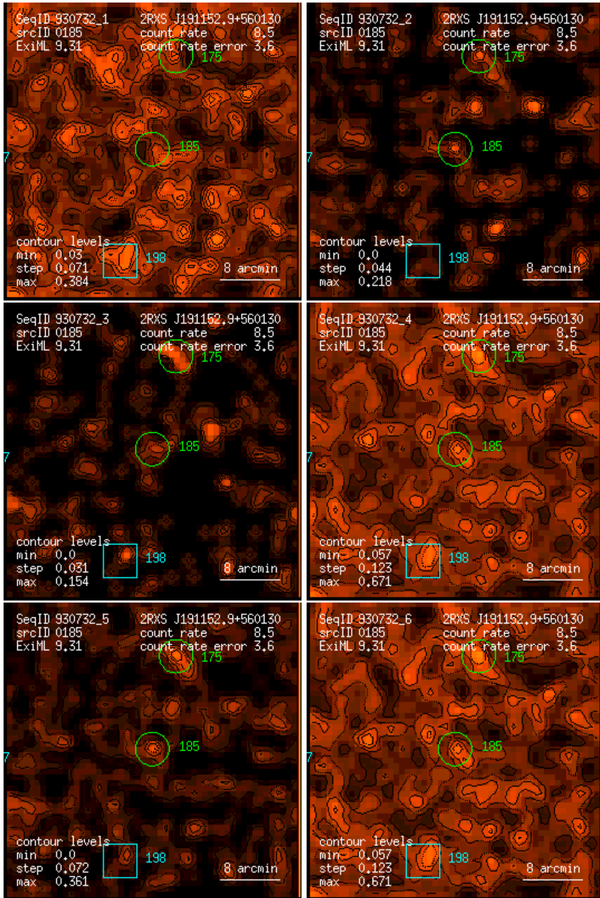
Figure 185: RASS 930732: detection 0185: band rate images, Gaussian filter: (1) PSPC channels 11 – 41, (2) 52 – 90, (3) 91 – 201, (4) 11 – 235, (5) 52 – 201, (6) 11 – 201. Broad band rates in counts/ks. Band rate contour levels in counts/ks/arcmin 2 .
