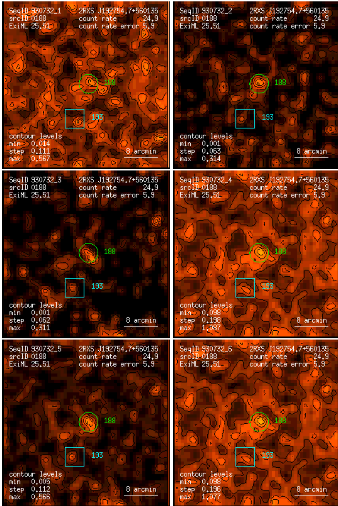
Figure 188: RASS 930732: detection 0188: band rate images, Gaussian filter: (1) PSPC channels 11 – 41, (2) 52 – 90, (3) 91 – 201, (4) 11 – 235, (5) 52 – 201, (6) 11 – 201. Broad band rates in counts/ks. Band rate contour levels in counts/ks/arcmin 2 .
