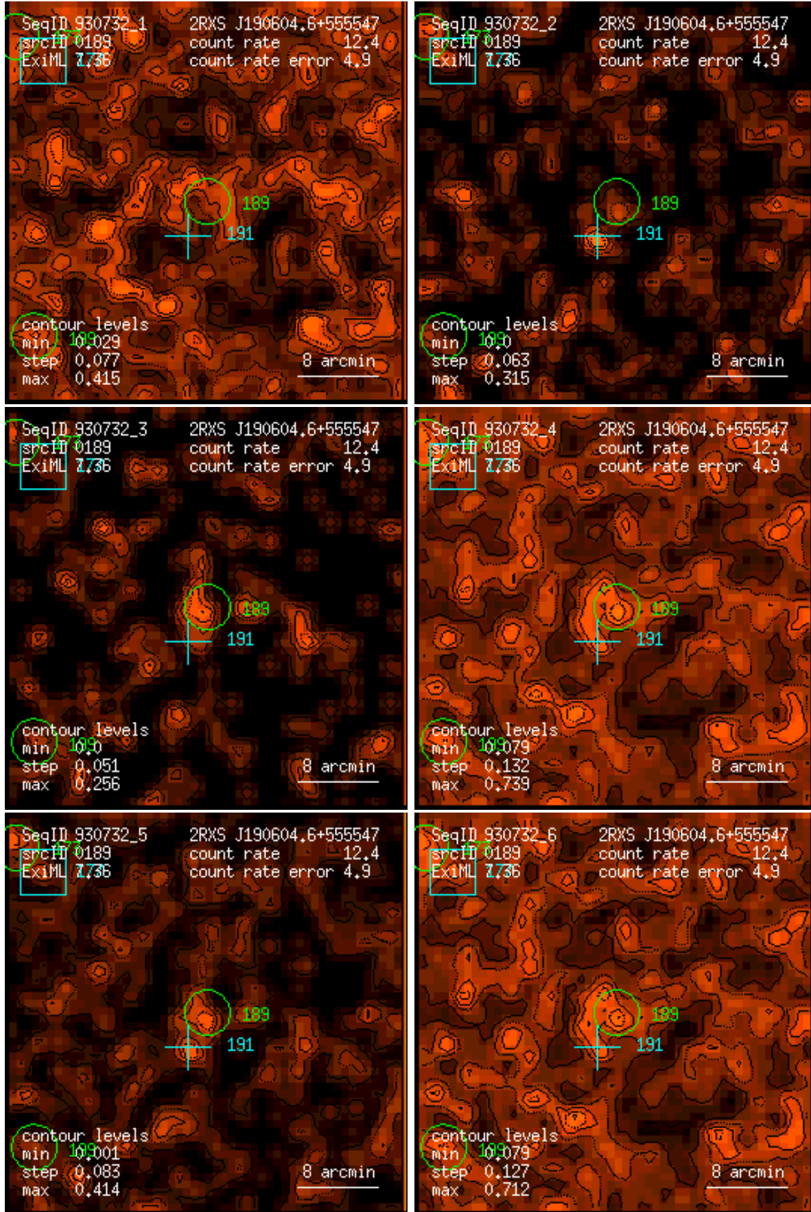
Figure 189: RASS 930732: detection 0189: band rate images, Gaussian filter: (1) PSPC channels 11 – 41, (2) 52 – 90, (3) 91 – 201, (4) 11 – 235, (5) 52 – 201, (6) 11 – 201. Broad band rates in counts/ks. Band rate contour levels in counts/ks/arcmin 2 .
