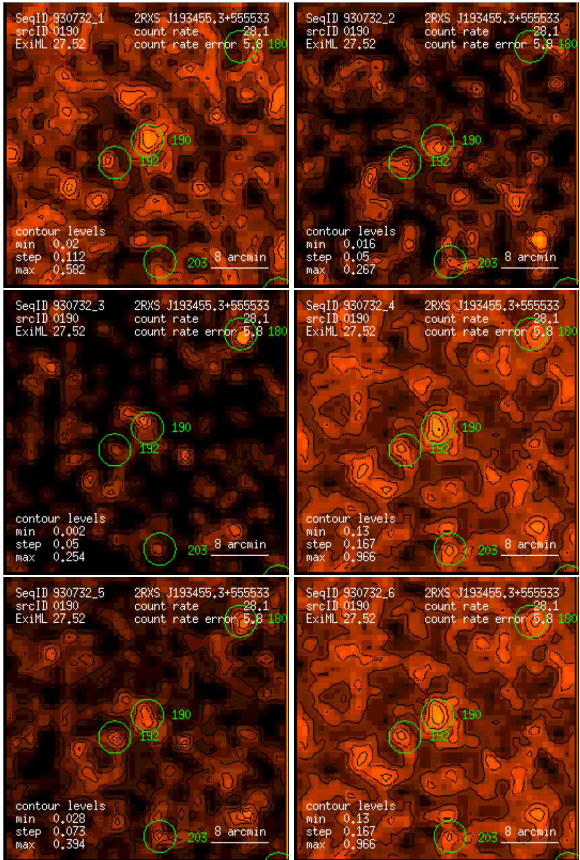
Figure 190: RASS 930732: detection 0190: band rate images, Gaussian filter: (1) PSPC channels 11 – 41, (2) 52 – 90, (3) 91 – 201, (4) 11 – 235, (5) 52 – 201, (6) 11 – 201. Broad band rates in counts/ks. Band rate contour levels in counts/ks/arcmin 2 .
