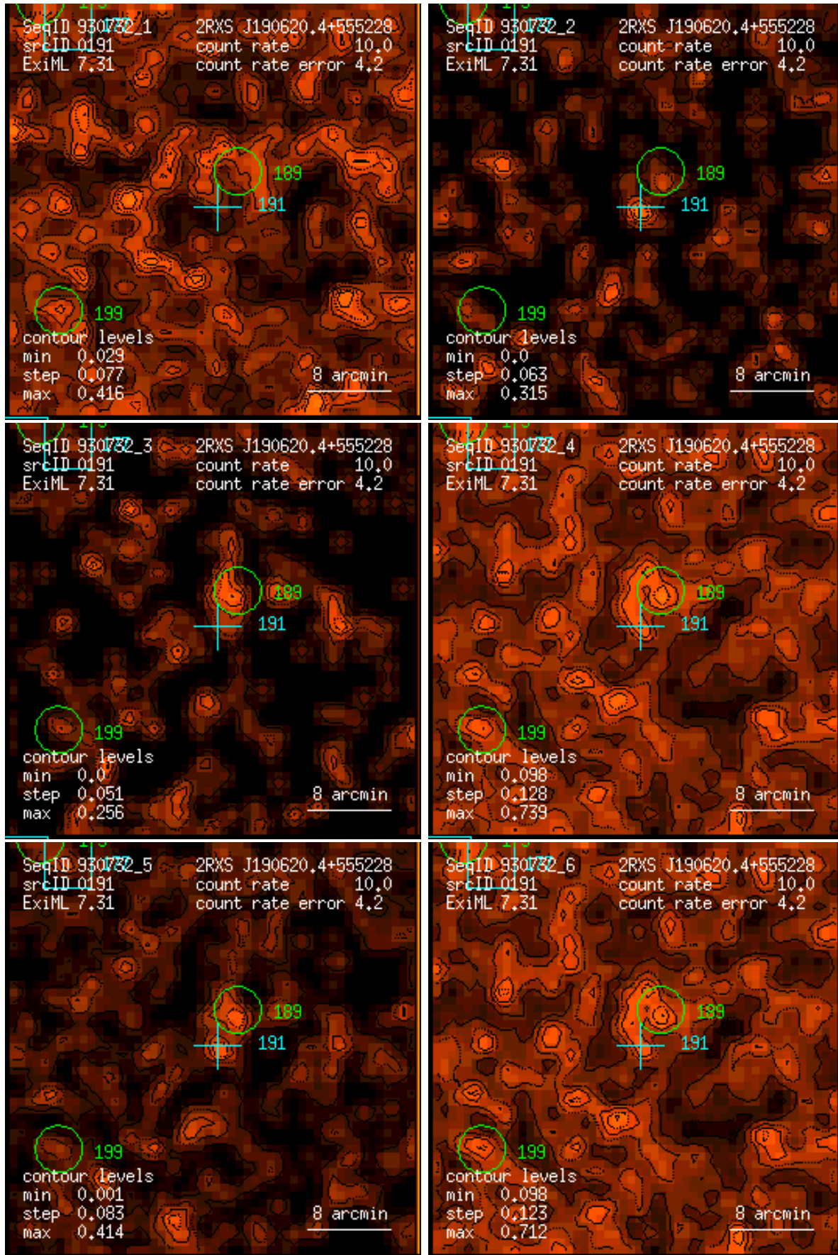
Figure 191: RASS 930732: detection 0191: band rate images, Gaussian filter: (1) PSPC channels 11 – 41, (2) 52 – 90, (3) 91 – 201, (4) 11 – 235, (5) 52 – 201, (6) 11 – 201. Broad band rates in counts/ks. Band rate contour levels in counts/ks/arcmin 2 .
