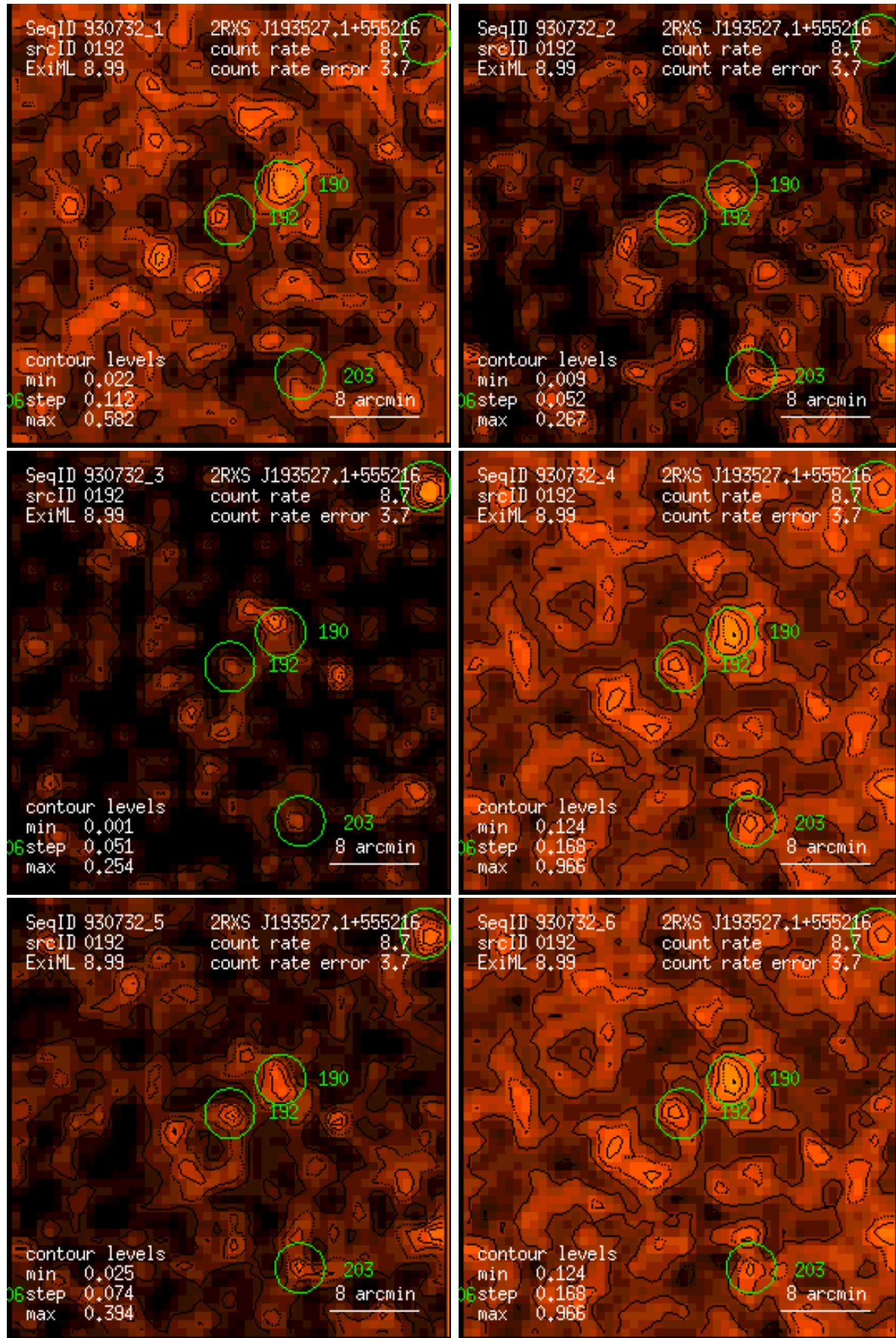
Figure 192: RASS 930732: detection 0192: band rate images, Gaussian filter: (1) PSPC channels 11 – 41, (2) 52 – 90, (3) 91 – 201, (4) 11 – 235, (5) 52 – 201, (6) 11 – 201. Broad band rates in counts/ks. Band rate contour levels in counts/ks/arcmin 2 .
