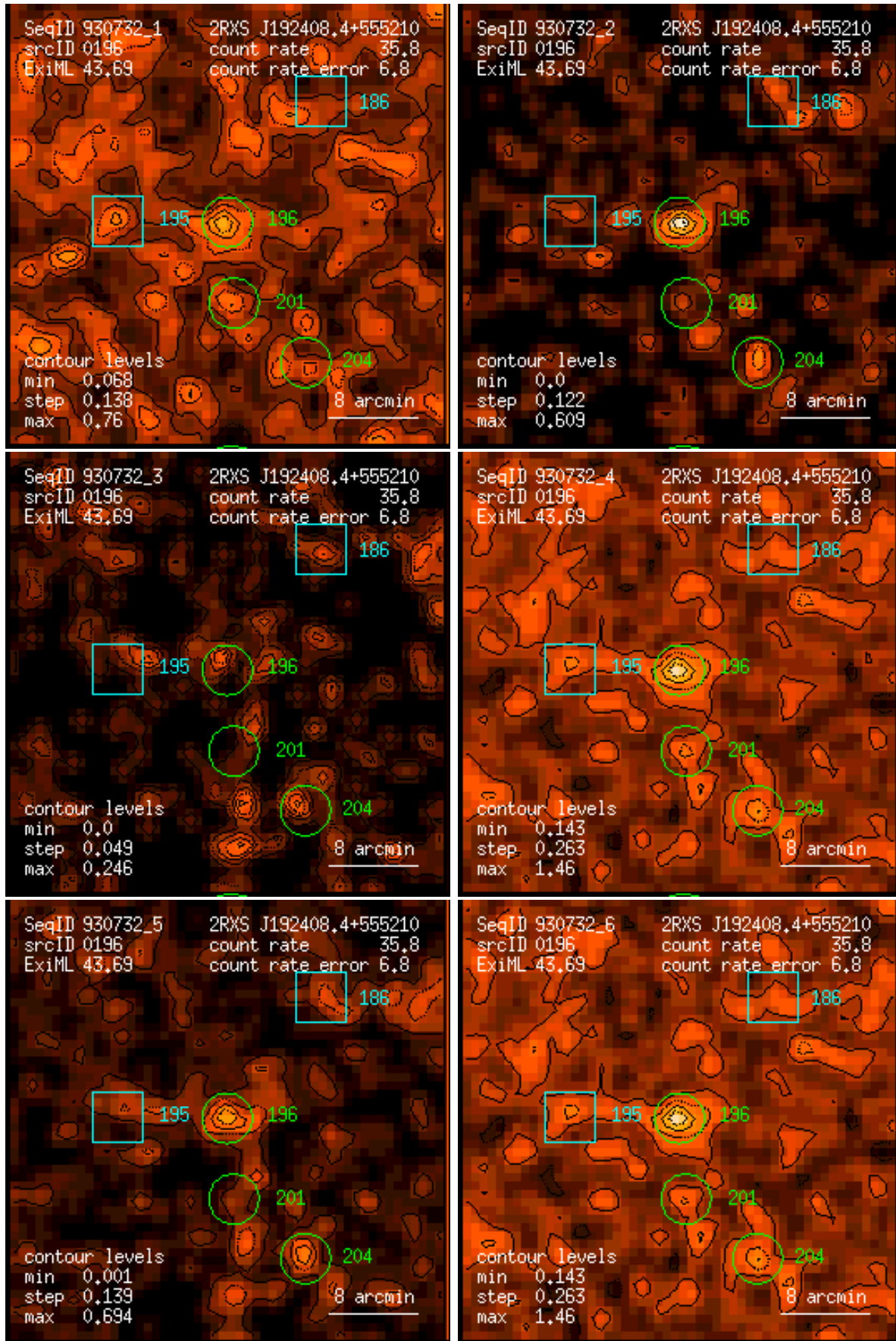
Figure 196: RASS 930732: detection 0196: band rate images, Gaussian filter: (1) PSPC channels 11 – 41, (2) 52 – 90, (3) 91 – 201, (4) 11 – 235, (5) 52 – 201, (6) 11 – 201. Broad band rates in counts/ks. Band rate contour levels in counts/ks/arcmin 2 .
