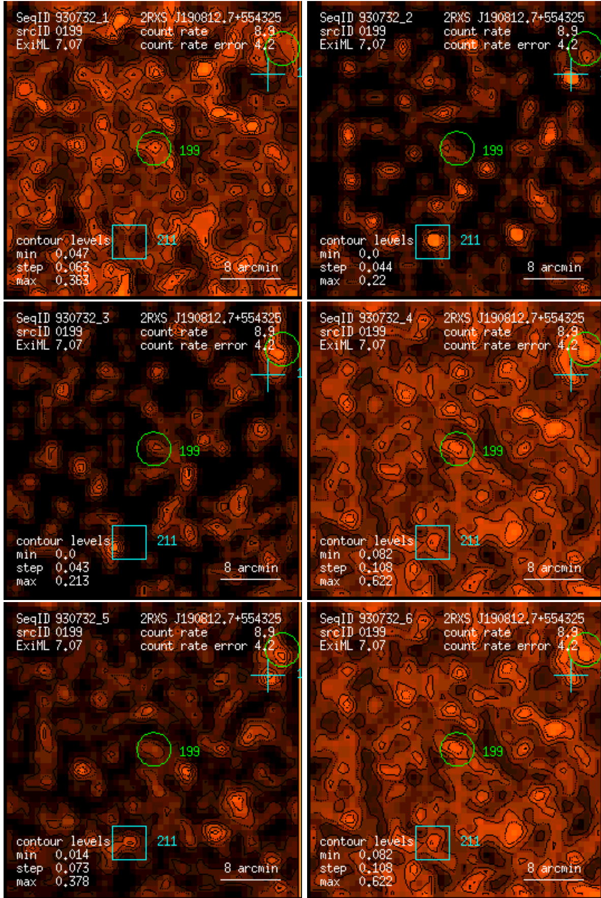
Figure 199: RASS 930732: detection 0199: band rate images, Gaussian filter: (1) PSPC channels 11 – 41, (2) 52 – 90, (3) 91 – 201, (4) 11 – 235, (5) 52 – 201, (6) 11 – 201. Broad band rates in counts/ks. Band rate contour levels in counts/ks/arcmin 2 .
