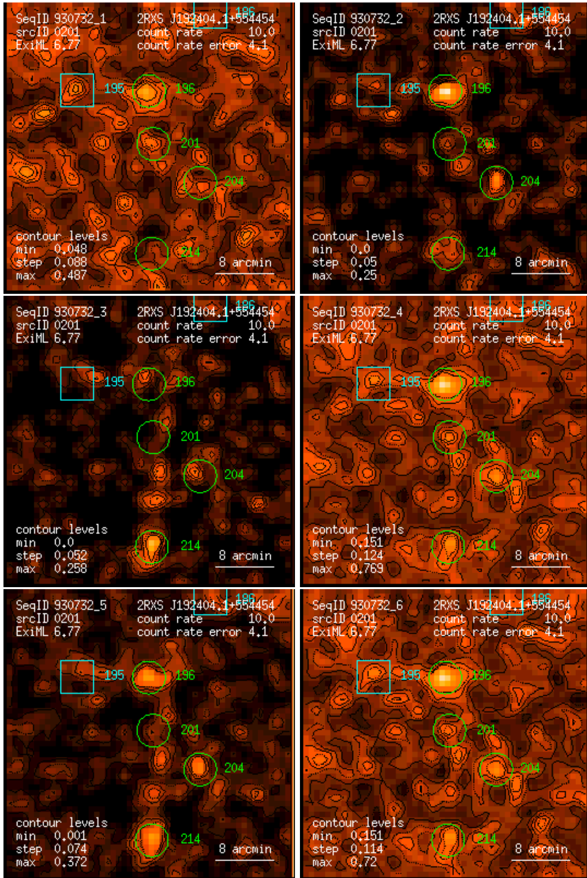
Figure 201: RASS 930732: detection 0201: band rate images, Gaussian filter: (1) PSPC channels 11 – 41, (2) 52 – 90, (3) 91 – 201, (4) 11 – 235, (5) 52 – 201, (6) 11 – 201. Broad band rates in counts/ks. Band rate contour levels in counts/ks/arcmin 2 .
