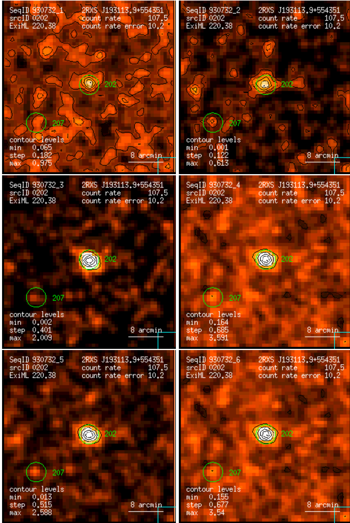
Figure 202: RASS 930732: detection 0202: band rate images, Gaussian filter: (1) PSPC channels 11 – 41, (2) 52 – 90, (3) 91 – 201, (4) 11 – 235, (5) 52 – 201, (6) 11 – 201. Broad band rates in counts/ks. Band rate contour levels in counts/ks/arcmin 2 .
