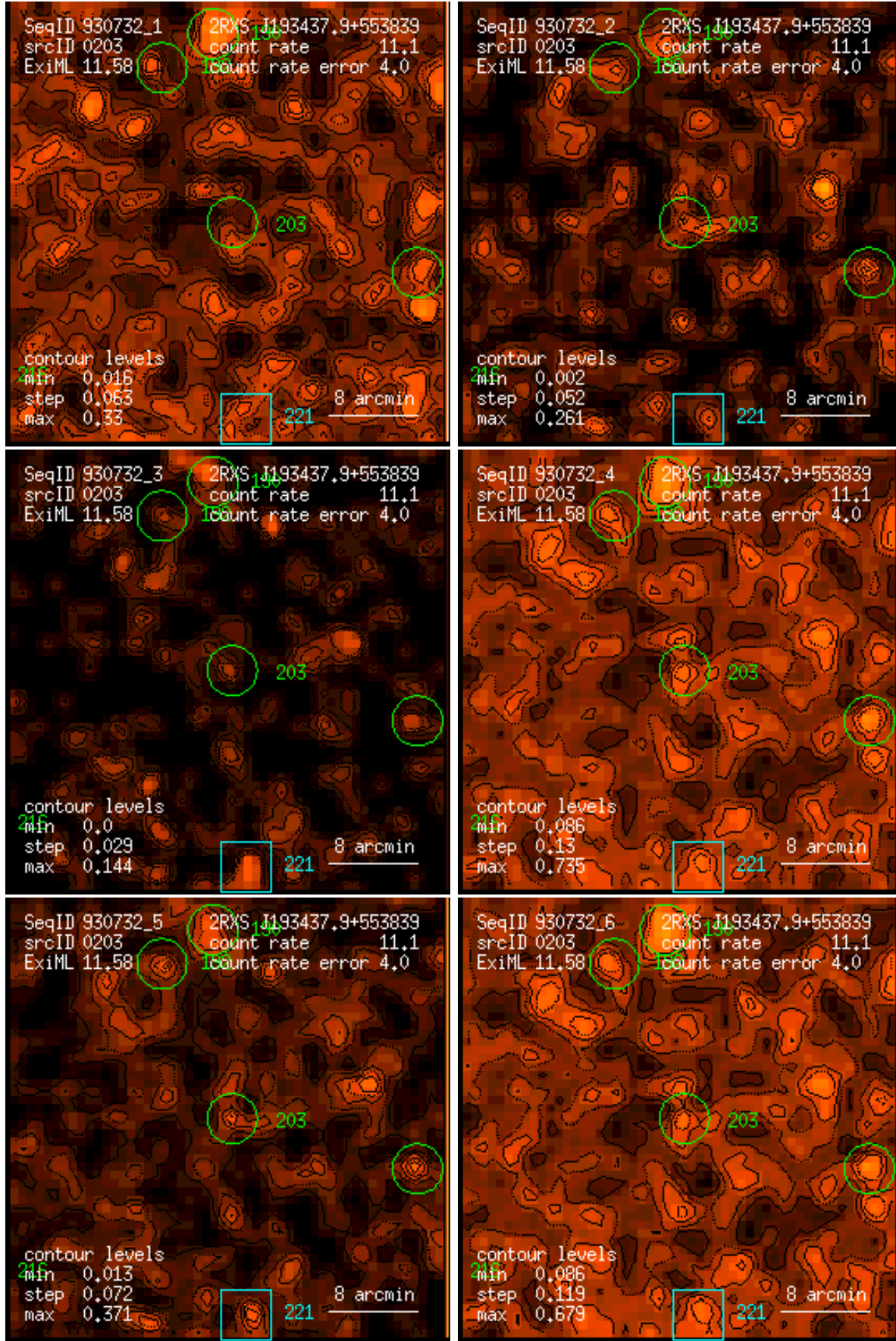
Figure 203: RASS 930732: detection 0203: band rate images, Gaussian filter: (1) PSPC channels 11 – 41, (2) 52 – 90, (3) 91 – 201, (4) 11 – 235, (5) 52 – 201, (6) 11 – 201. Broad band rates in counts/ks. Band rate contour levels in counts/ks/arcmin 2 .
