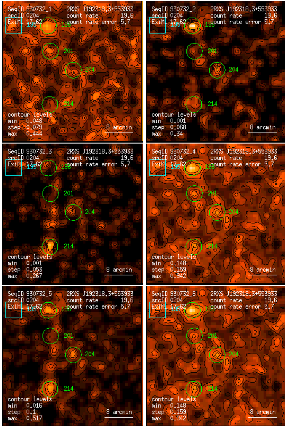
Figure 204: RASS 930732: detection 0204: band rate images, Gaussian filter: (1) PSPC channels 11 – 41, (2) 52 – 90, (3) 91 – 201, (4) 11 – 235, (5) 52 – 201, (6) 11 – 201. Broad band rates in counts/ks. Band rate contour levels in counts/ks/arcmin 2 .
