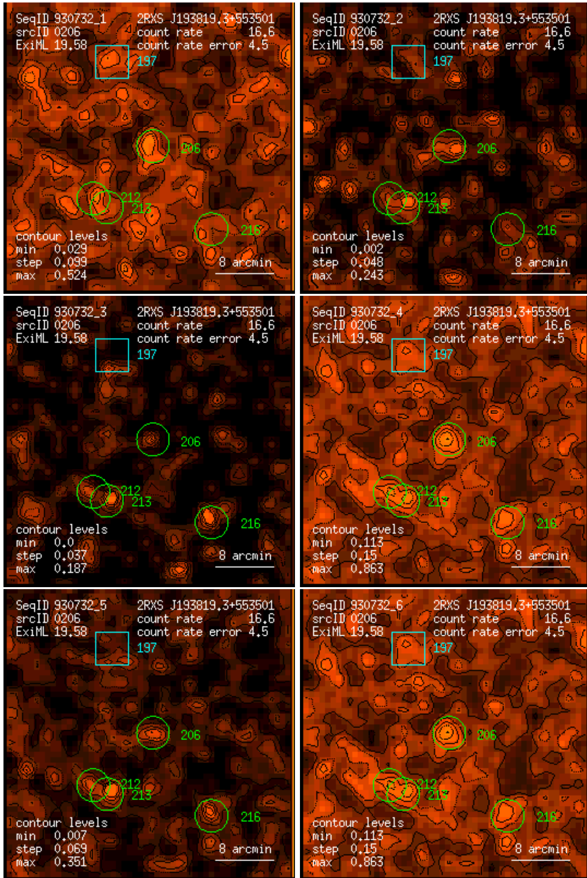
Figure 206: RASS 930732: detection 0206: band rate images, Gaussian filter: (1) PSPC channels 11 – 41, (2) 52 – 90, (3) 91 – 201, (4) 11 – 235, (5) 52 – 201, (6) 11 – 201. Broad band rates in counts/ks. Band rate contour levels in counts/ks/arcmin 2 .
