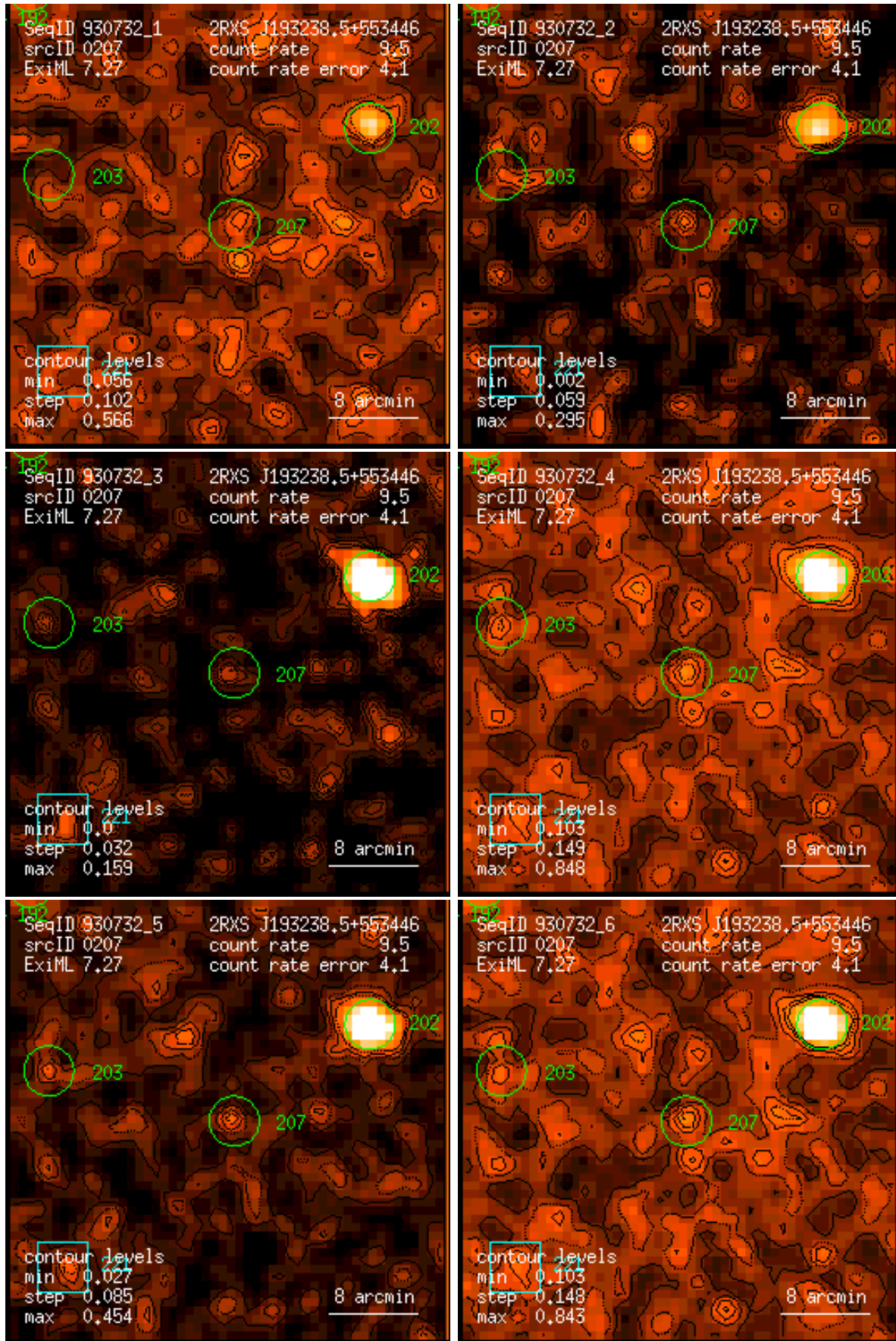
Figure 207: RASS 930732: detection 0207: band rate images, Gaussian filter: (1) PSPC channels 11 – 41, (2) 52 – 90, (3) 91 – 201, (4) 11 – 235, (5) 52 – 201, (6) 11 – 201. Broad band rates in counts/ks. Band rate contour levels in counts/ks/arcmin 2 .
