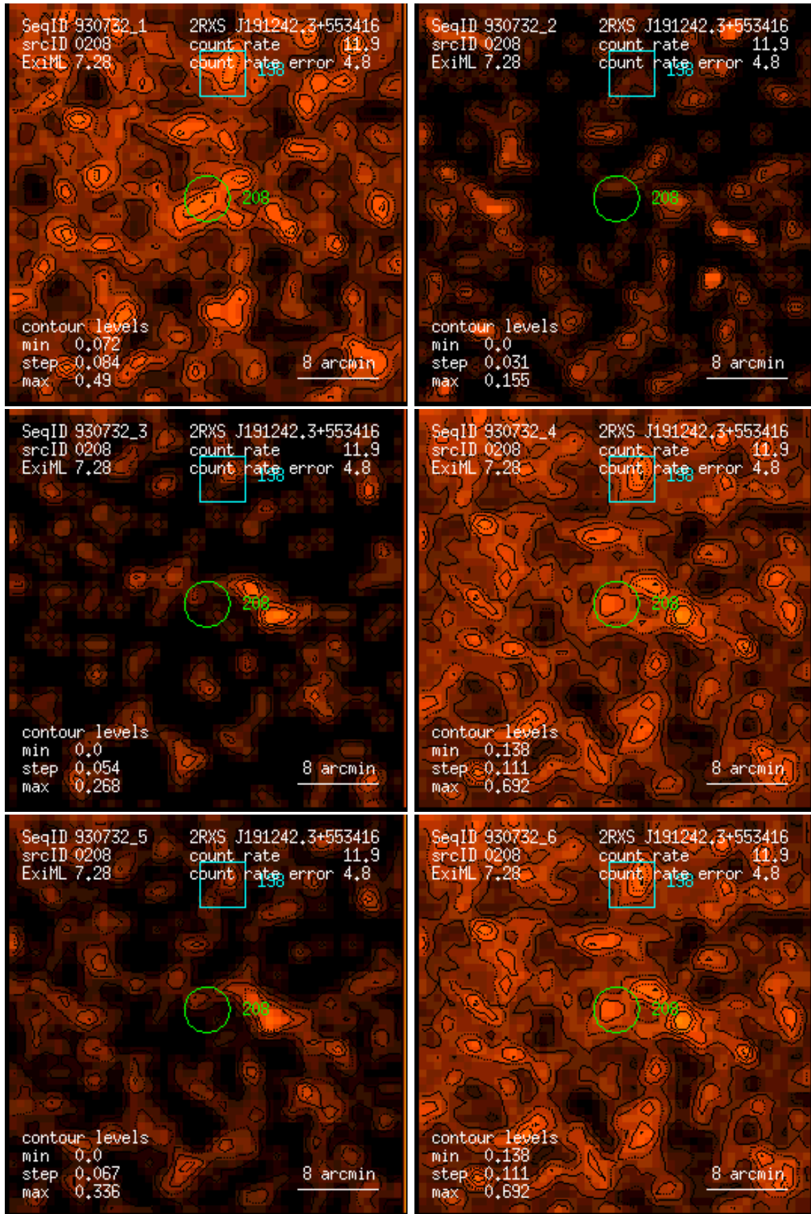
Figure 208: RASS 930732: detection 0208: band rate images, Gaussian filter: (1) PSPC channels 11 – 41, (2) 52 – 90, (3) 91 – 201, (4) 11 – 235, (5) 52 – 201, (6) 11 – 201. Broad band rates in counts/ks. Band rate contour levels in counts/ks/arcmin 2 .
