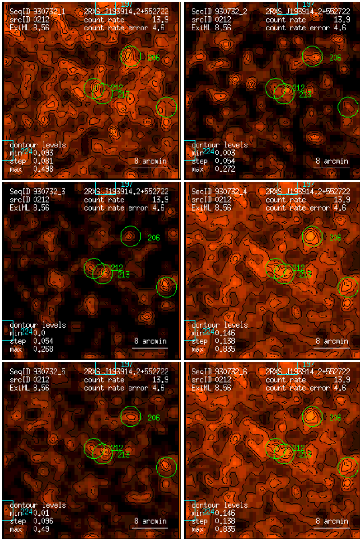
Figure 212: RASS 930732: detection 0212: band rate images, Gaussian filter: (1) PSPC channels 11 – 41, (2) 52 – 90, (3) 91 – 201, (4) 11 – 235, (5) 52 – 201, (6) 11 – 201. Broad band rates in counts/ks. Band rate contour levels in counts/ks/arcmin 2 .
