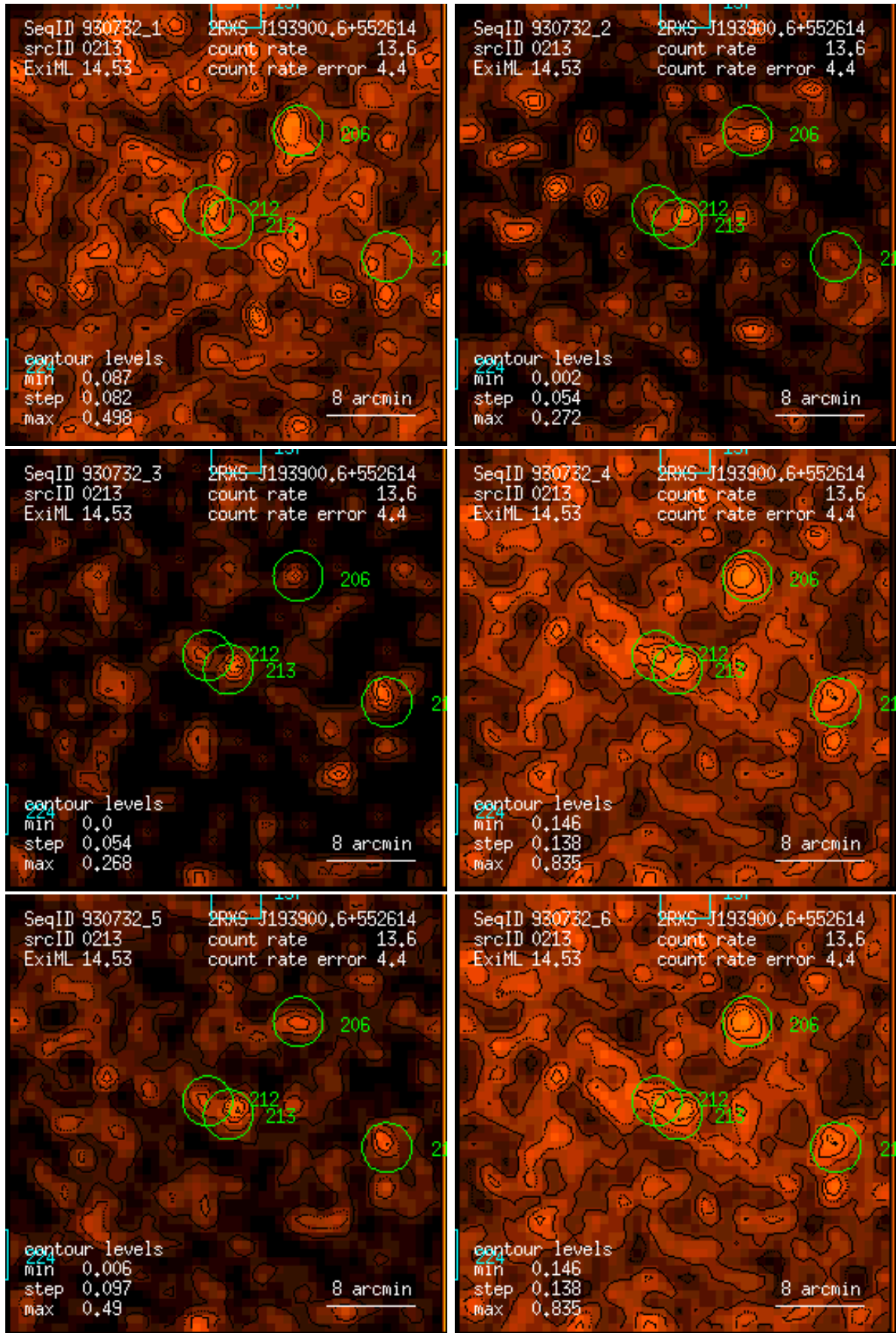
Figure 213: RASS 930732: detection 0213: band rate images, Gaussian filter: (1) PSPC channels 11 – 41, (2) 52 – 90, (3) 91 – 201, (4) 11 – 235, (5) 52 – 201, (6) 11 – 201. Broad band rates in counts/ks. Band rate contour levels in counts/ks/arcmin 2 .
