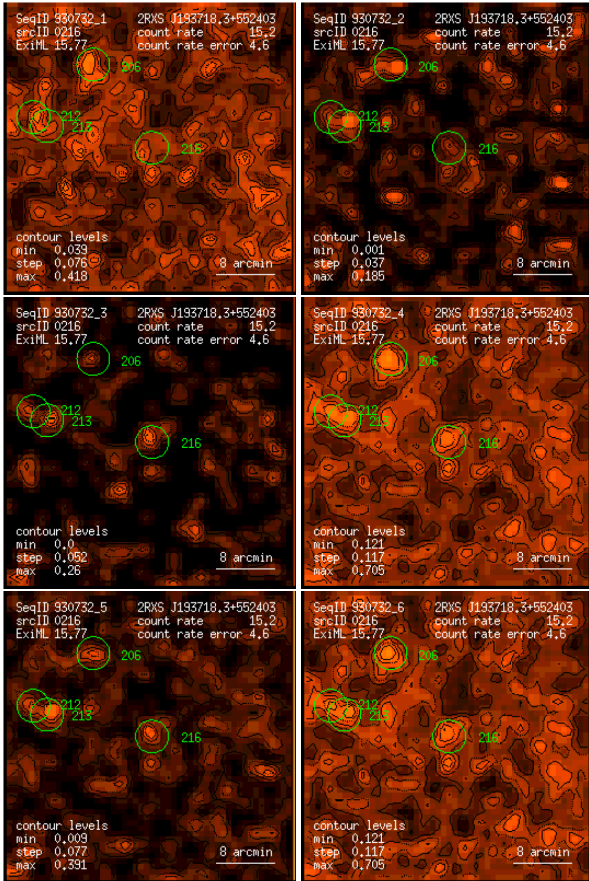
Figure 216: RASS 930732: detection 0216: band rate images, Gaussian filter: (1) PSPC channels 11 – 41, (2) 52 – 90, (3) 91 – 201, (4) 11 – 235, (5) 52 – 201, (6) 11 – 201. Broad band rates in counts/ks. Band rate contour levels in counts/ks/arcmin 2 .
