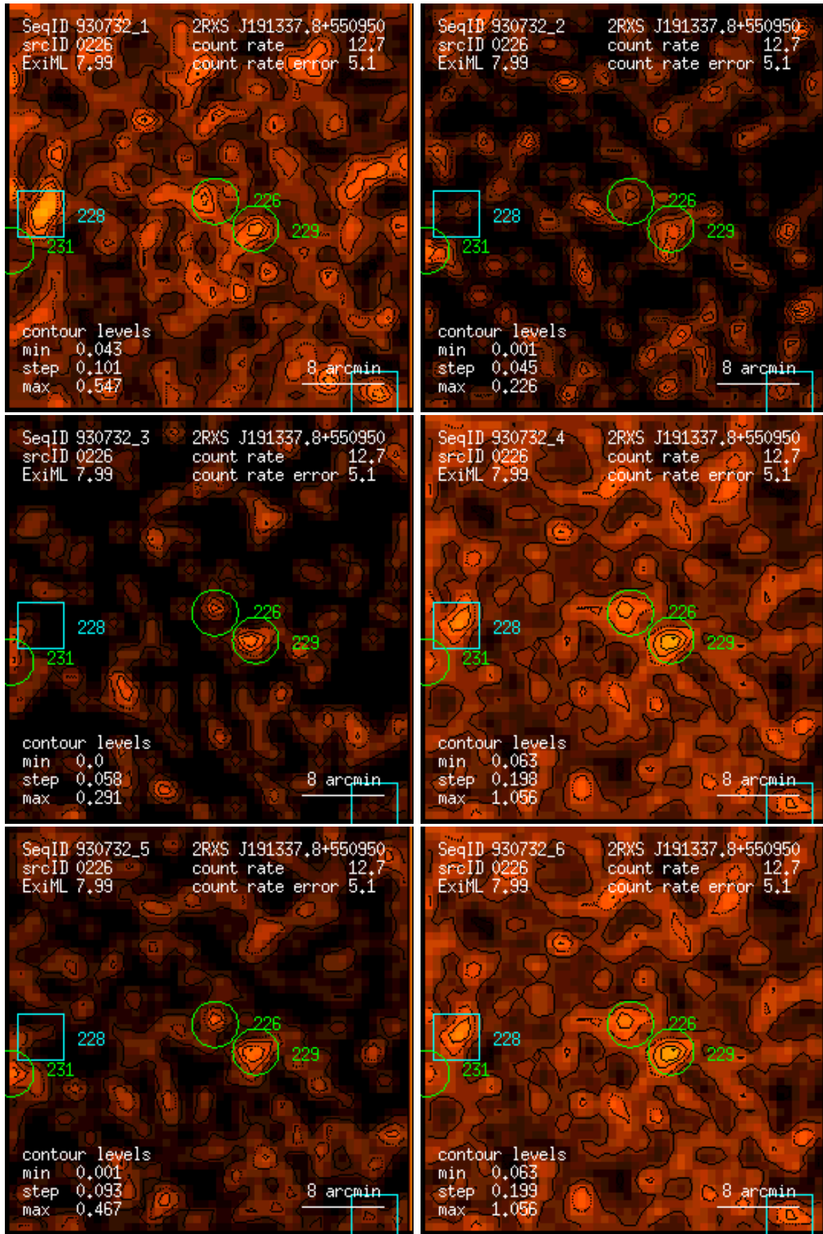
Figure 226: RASS 930732: detection 0226: band rate images, Gaussian filter: (1) PSPC channels 11 – 41, (2) 52 – 90, (3) 91 – 201, (4) 11 – 235, (5) 52 – 201, (6) 11 – 201. Broad band rates in counts/ks. Band rate contour levels in counts/ks/arcmin 2 .
