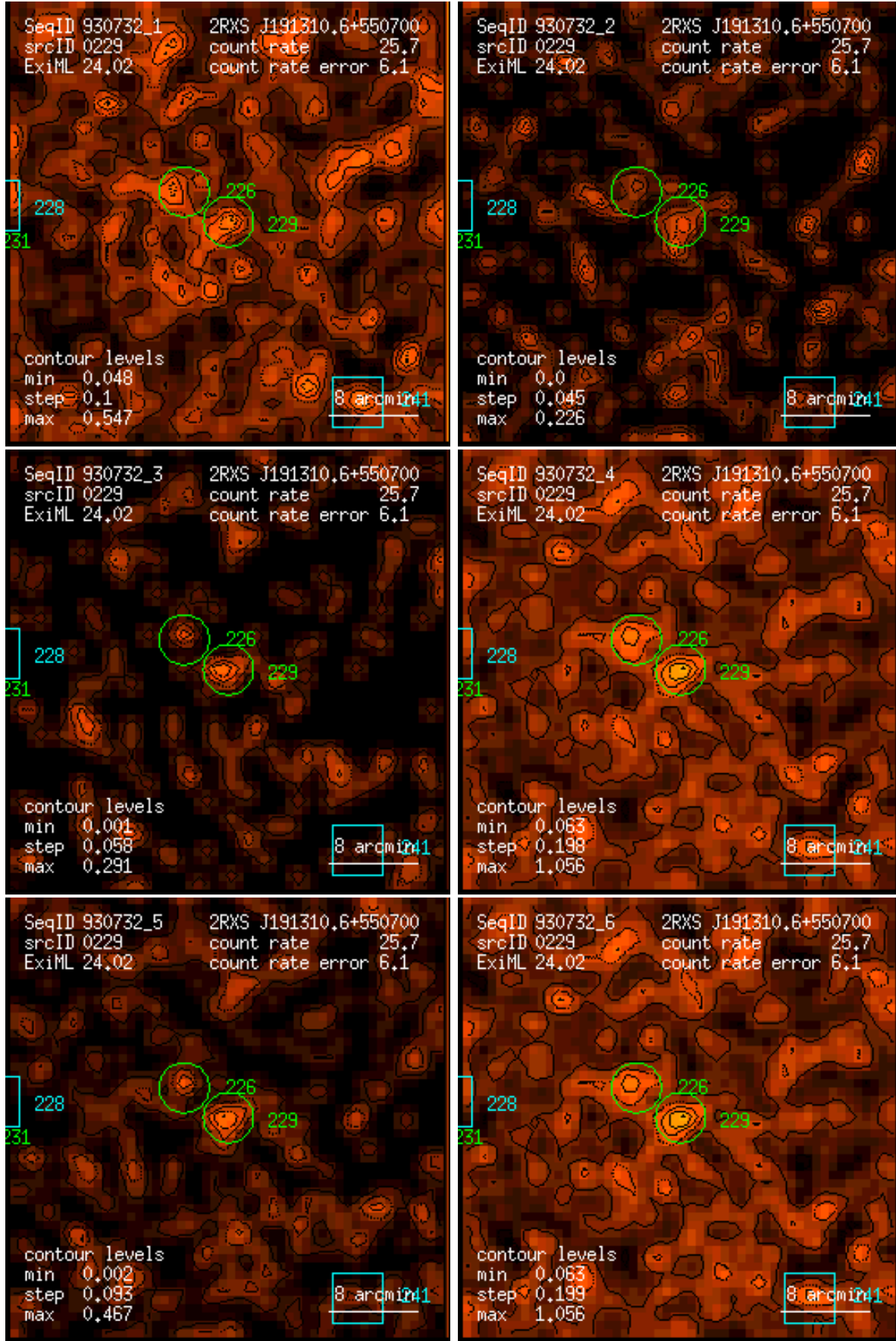
Figure 229: RASS 930732: detection 0229: band rate images, Gaussian filter: (1) PSPC channels 11 – 41, (2) 52 – 90, (3) 91 – 201, (4) 11 – 235, (5) 52 – 201, (6) 11 – 201. Broad band rates in counts/ks. Band rate contour levels in counts/ks/arcmin 2 .
