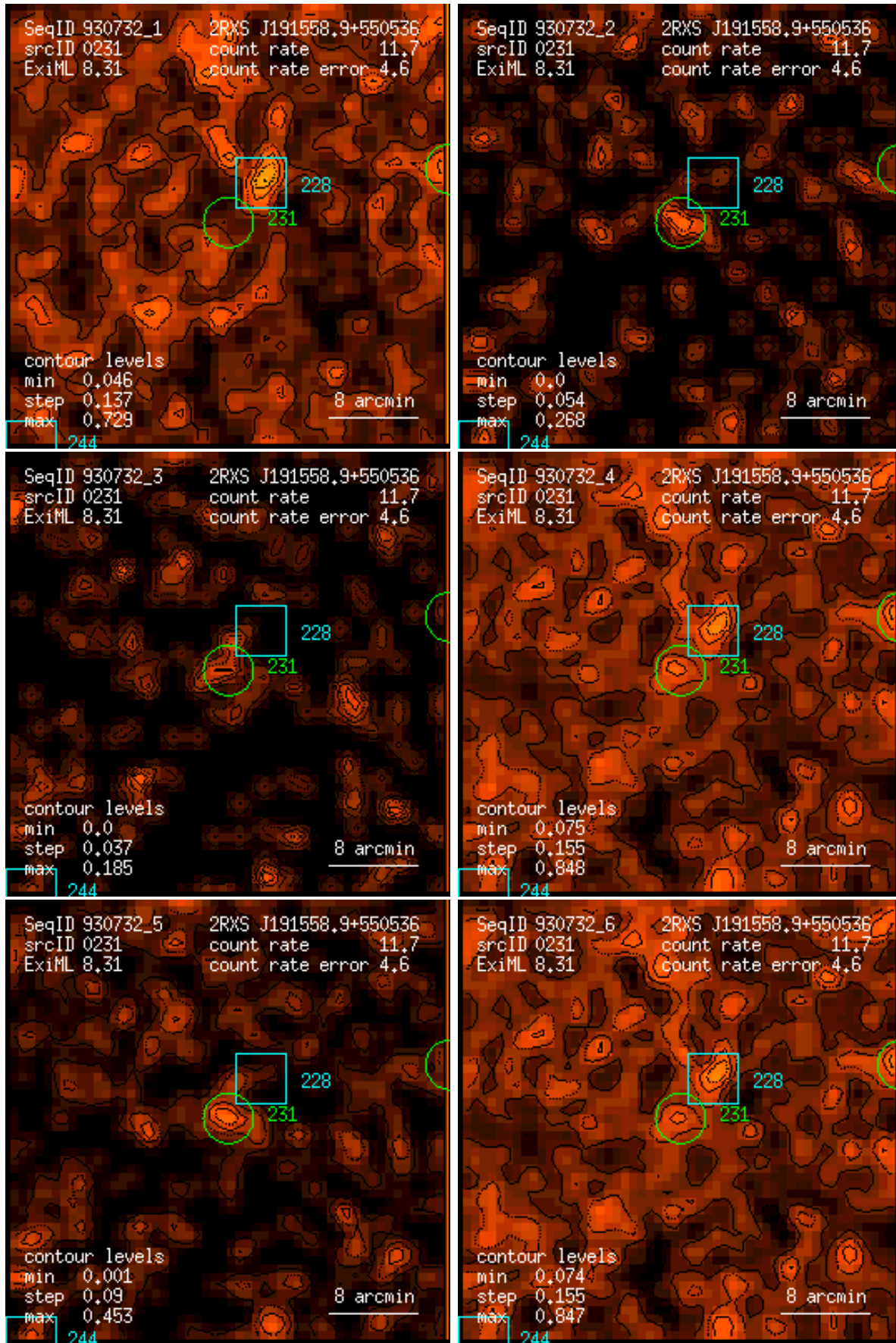
Figure 231: RASS 930732: detection 0231: band rate images, Gaussian filter: (1) PSPC channels 11 – 41, (2) 52 – 90, (3) 91 – 201, (4) 11 – 235, (5) 52 – 201, (6) 11 – 201. Broad band rates in counts/ks. Band rate contour levels in counts/ks/arcmin 2 .
