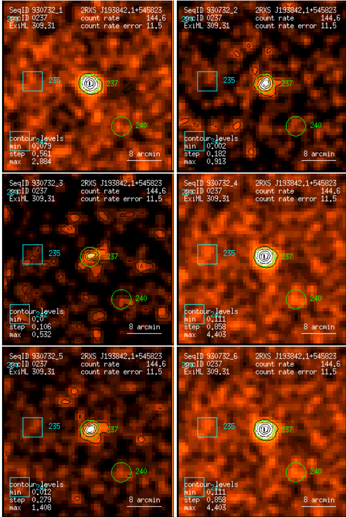
Figure 237: RASS 930732: detection 0237: band rate images, Gaussian filter: (1) PSPC channels 11 – 41, (2) 52 – 90, (3) 91 – 201, (4) 11 – 235, (5) 52 – 201, (6) 11 – 201. Broad band rates in counts/ks. Band rate contour levels in counts/ks/arcmin 2 .
