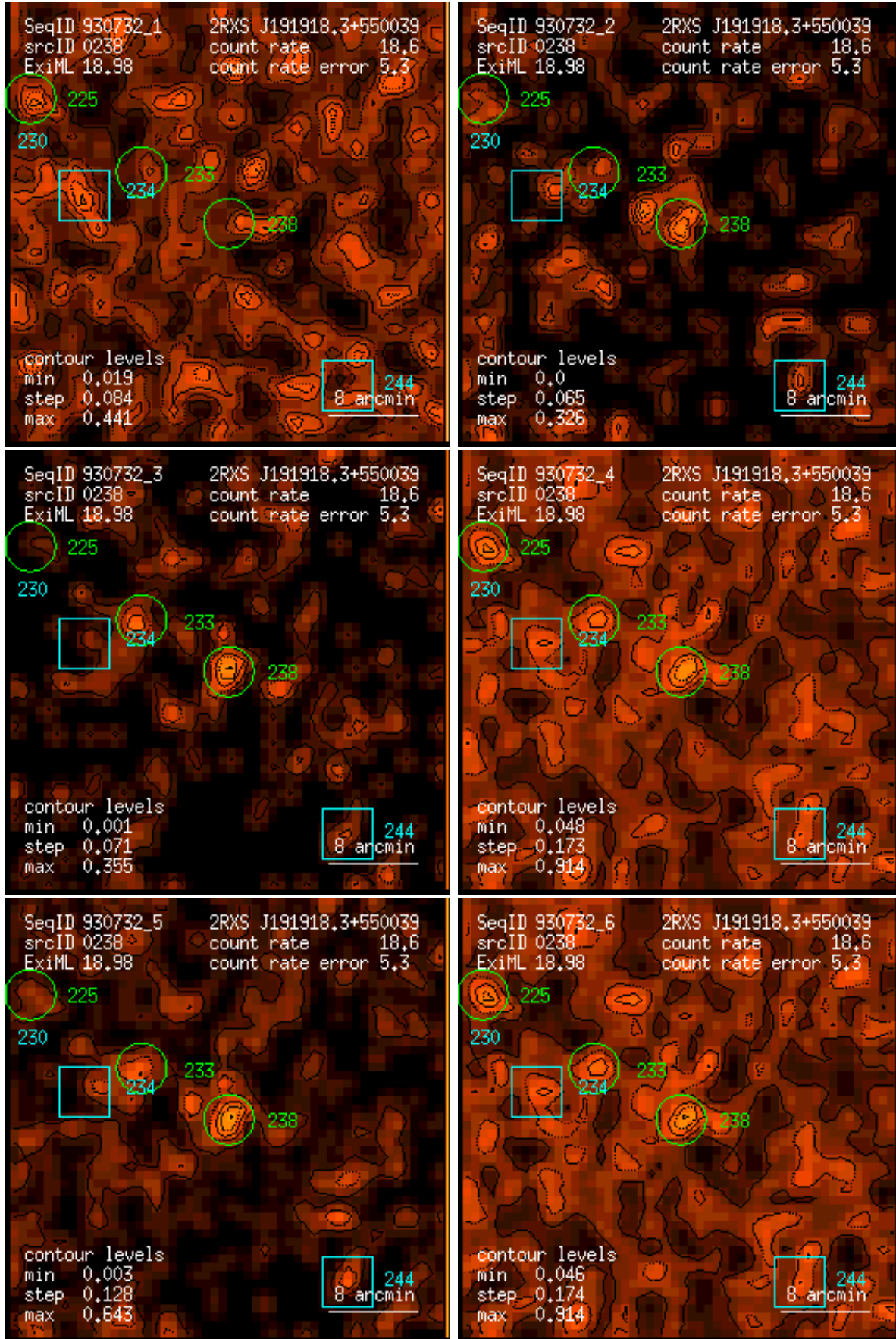
Figure 238: RASS 930732: detection 0238: band rate images, Gaussian filter: (1) PSPC channels 11 – 41, (2) 52 – 90, (3) 91 – 201, (4) 11 – 235, (5) 52 – 201, (6) 11 – 201. Broad band rates in counts/ks. Band rate contour levels in counts/ks/arcmin 2 .
