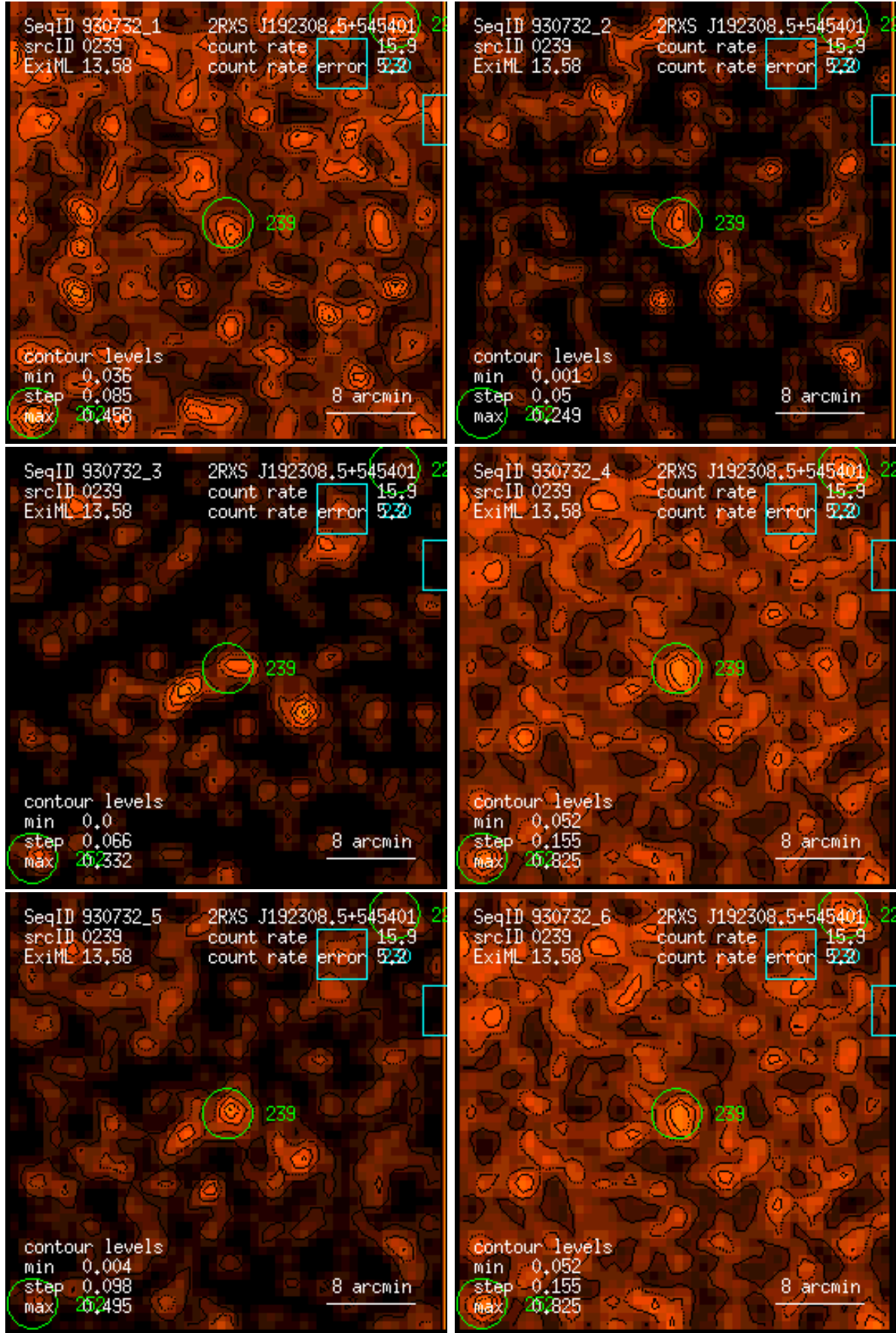
Figure 239: RASS 930732: detection 0239: band rate images, Gaussian filter: (1) PSPC channels 11 – 41, (2) 52 – 90, (3) 91 – 201, (4) 11 – 235, (5) 52 – 201, (6) 11 – 201. Broad band rates in counts/ks. Band rate contour levels in counts/ks/arcmin 2 .
