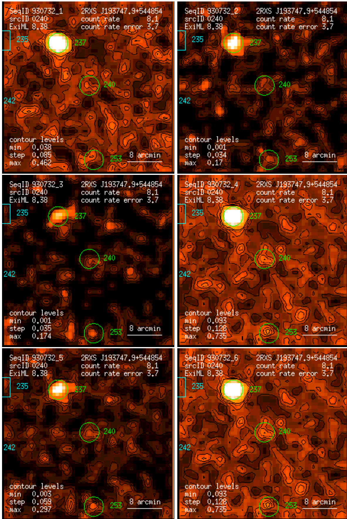
Figure 240: RASS 930732: detection 0240: band rate images, Gaussian filter: (1) PSPC channels 11 – 41, (2) 52 – 90, (3) 91 – 201, (4) 11 – 235, (5) 52 – 201, (6) 11 – 201. Broad band rates in counts/ks. Band rate contour levels in counts/ks/arcmin 2 .
