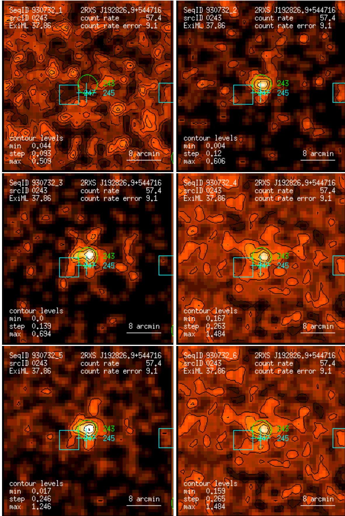
Figure 243: RASS 930732: detection 0243: band rate images, Gaussian filter: (1) PSPC channels 11 – 41, (2) 52 – 90, (3) 91 – 201, (4) 11 – 235, (5) 52 – 201, (6) 11 – 201. Broad band rates in counts/ks. Band rate contour levels in counts/ks/arcmin 2 .
