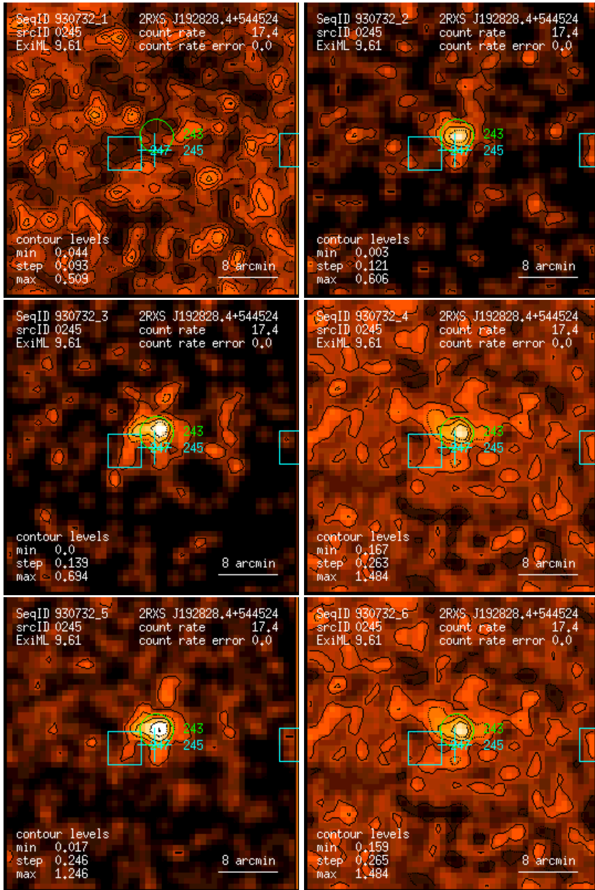
Figure 245: RASS 930732: detection 0245: band rate images, Gaussian filter: (1) PSPC channels 11 – 41, (2) 52 – 90, (3) 91 – 201, (4) 11 – 235, (5) 52 – 201, (6) 11 – 201. Broad band rates in counts/ks. Band rate contour levels in counts/ks/arcmin 2 .
