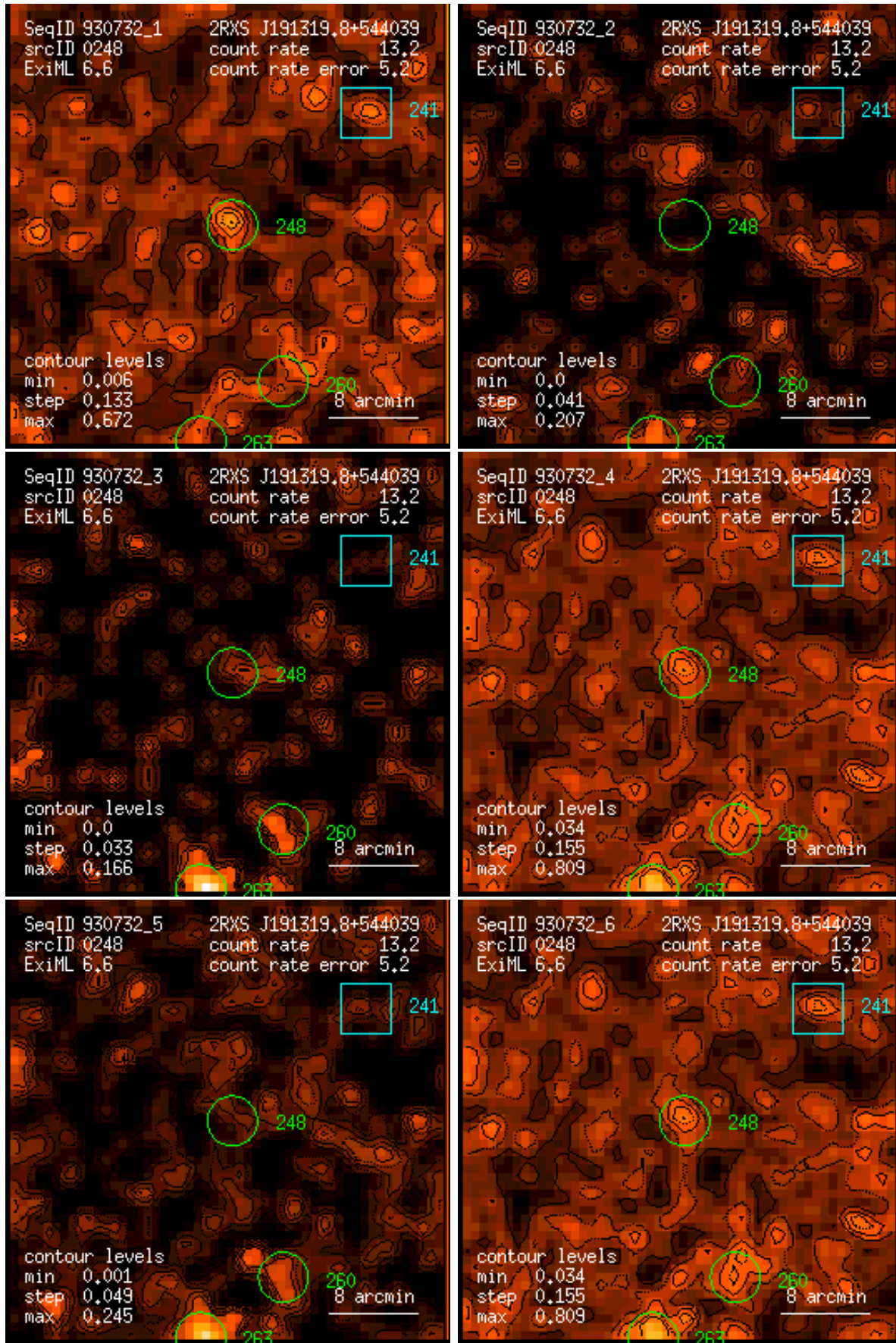
Figure 248: RASS 930732: detection 0248: band rate images, Gaussian filter: (1) PSPC channels 11 – 41, (2) 52 – 90, (3) 91 – 201, (4) 11 – 235, (5) 52 – 201, (6) 11 – 201. Broad band rates in counts/ks. Band rate contour levels in counts/ks/arcmin 2 .
