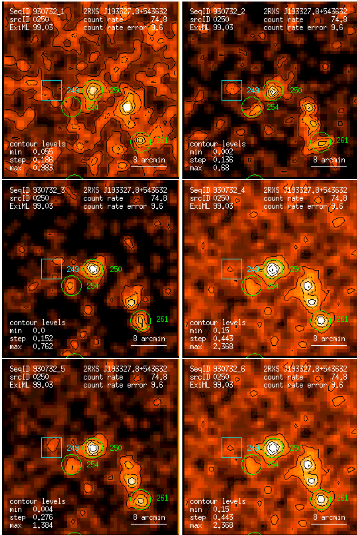
Figure 250: RASS 930732: detection 0250: band rate images, Gaussian filter: (1) PSPC channels 11 – 41, (2) 52 – 90, (3) 91 – 201, (4) 11 – 235, (5) 52 – 201, (6) 11 – 201. Broad band rates in counts/ks. Band rate contour levels in counts/ks/arcmin 2 .
