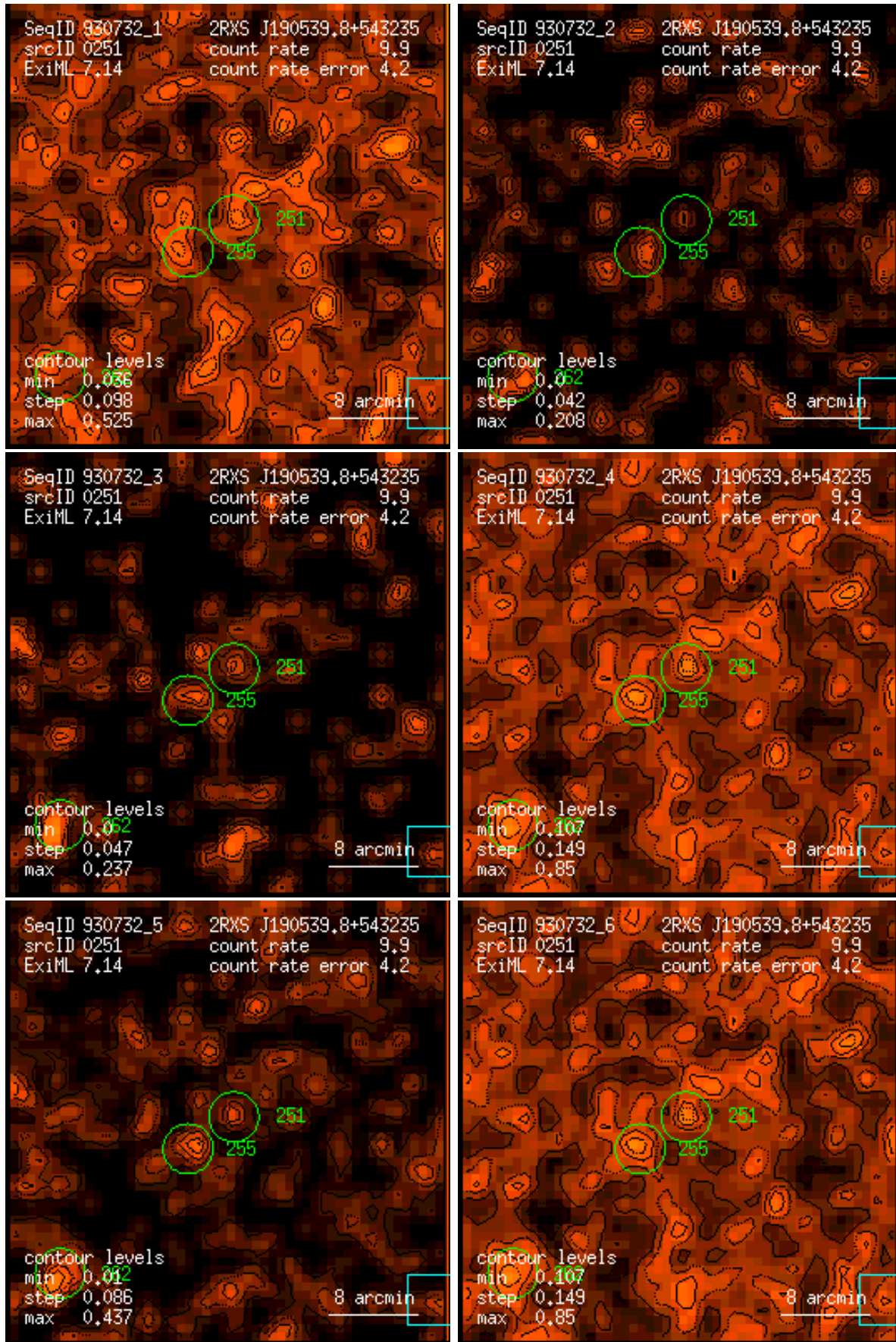
Figure 251: RASS 930732: detection 0251: band rate images, Gaussian filter: (1) PSPC channels 11 – 41, (2) 52 – 90, (3) 91 – 201, (4) 11 – 235, (5) 52 – 201, (6) 11 – 201. Broad band rates in counts/ks. Band rate contour levels in counts/ks/arcmin 2 .
