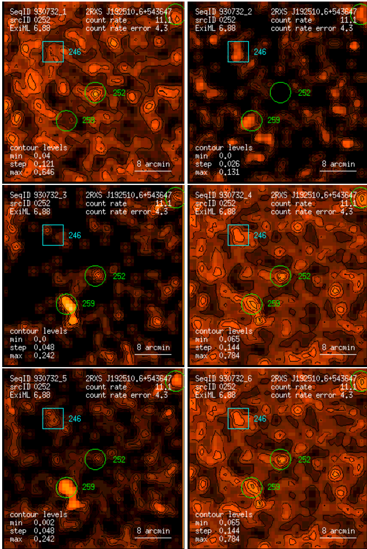
Figure 252: RASS 930732: detection 0252: band rate images, Gaussian filter: (1) PSPC channels 11 – 41, (2) 52 – 90, (3) 91 – 201, (4) 11 – 235, (5) 52 – 201, (6) 11 – 201. Broad band rates in counts/ks. Band rate contour levels in counts/ks/arcmin 2 .
