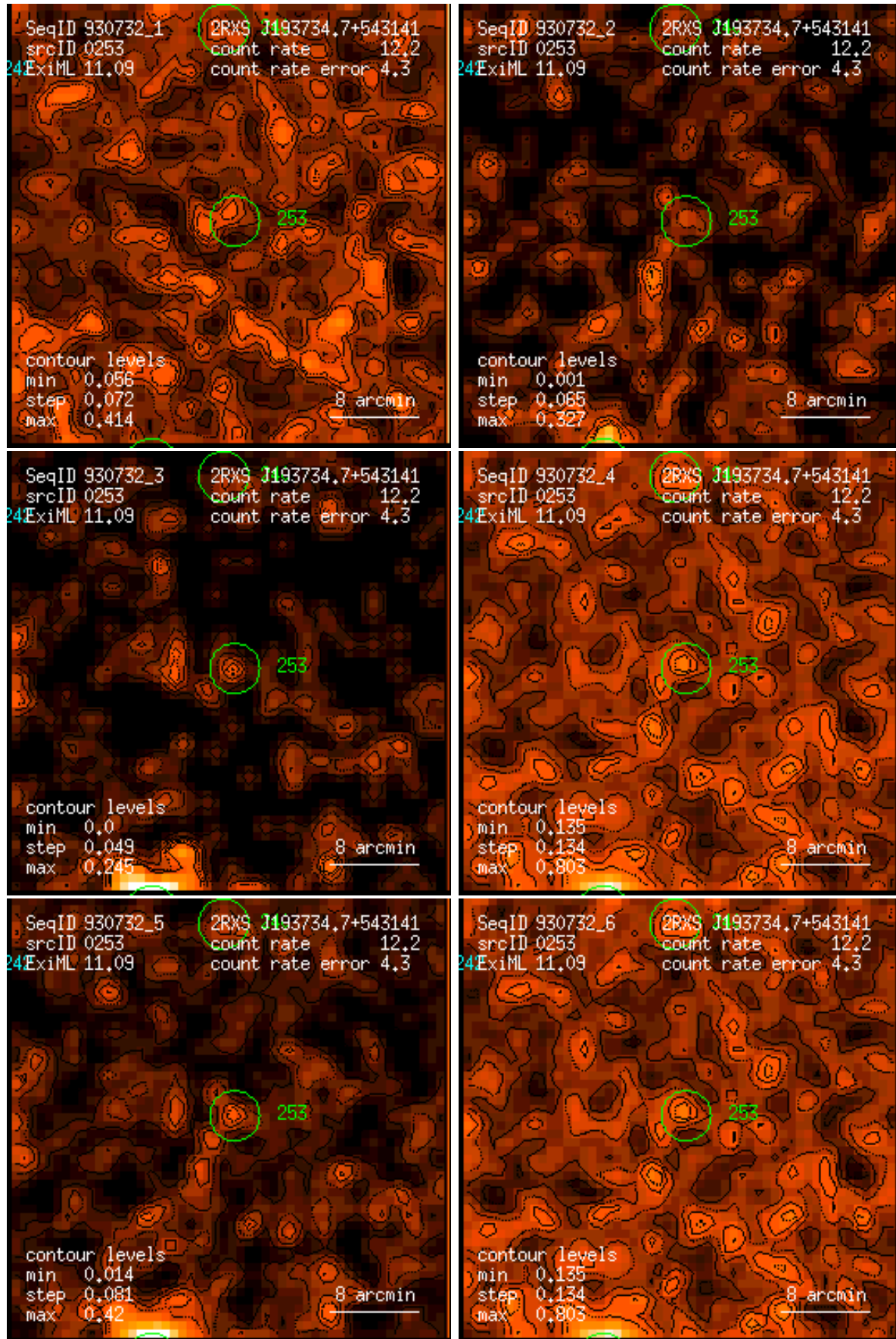
Figure 253: RASS 930732: detection 0253: band rate images, Gaussian filter: (1) PSPC channels 11 – 41, (2) 52 – 90, (3) 91 – 201, (4) 11 – 235, (5) 52 – 201, (6) 11 – 201. Broad band rates in counts/ks. Band rate contour levels in counts/ks/arcmin 2 .
