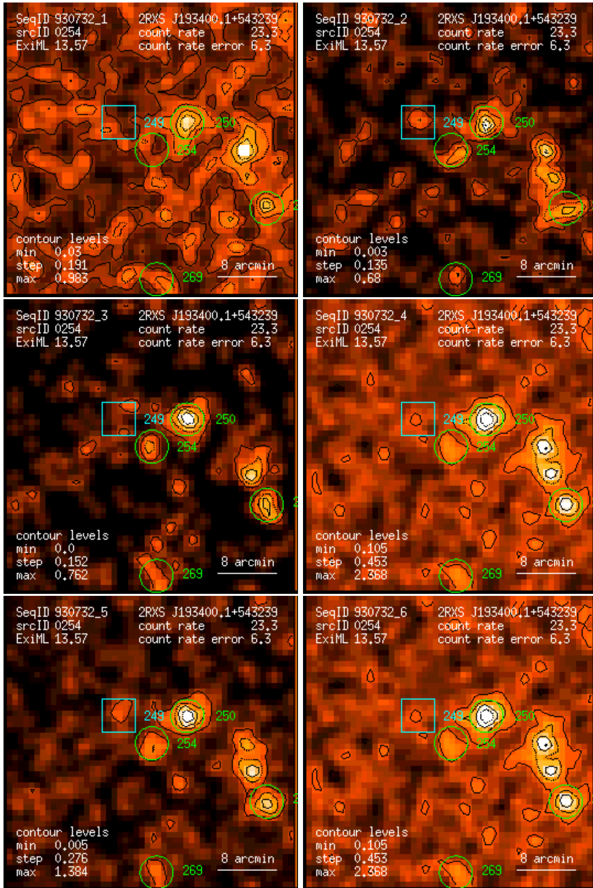
Figure 254: RASS 930732: detection 0254: band rate images, Gaussian filter: (1) PSPC channels 11 – 41, (2) 52 – 90, (3) 91 – 201, (4) 11 – 235, (5) 52 – 201, (6) 11 – 201. Broad band rates in counts/ks. Band rate contour levels in counts/ks/arcmin 2 .
