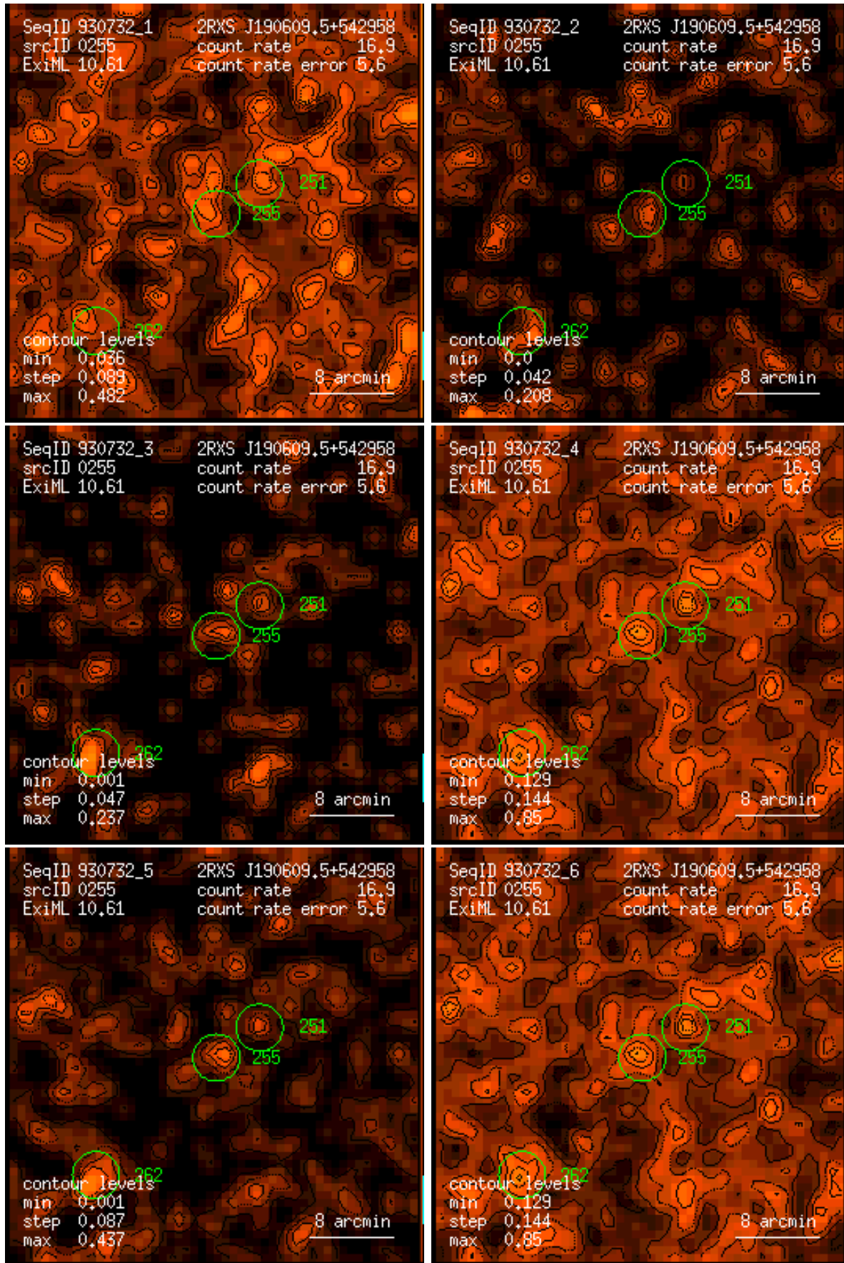
Figure 255: RASS 930732: detection 0255: band rate images, Gaussian filter: (1) PSPC channels 11 – 41, (2) 52 – 90, (3) 91 – 201, (4) 11 – 235, (5) 52 – 201, (6) 11 – 201. Broad band rates in counts/ks. Band rate contour levels in counts/ks/arcmin 2 .
