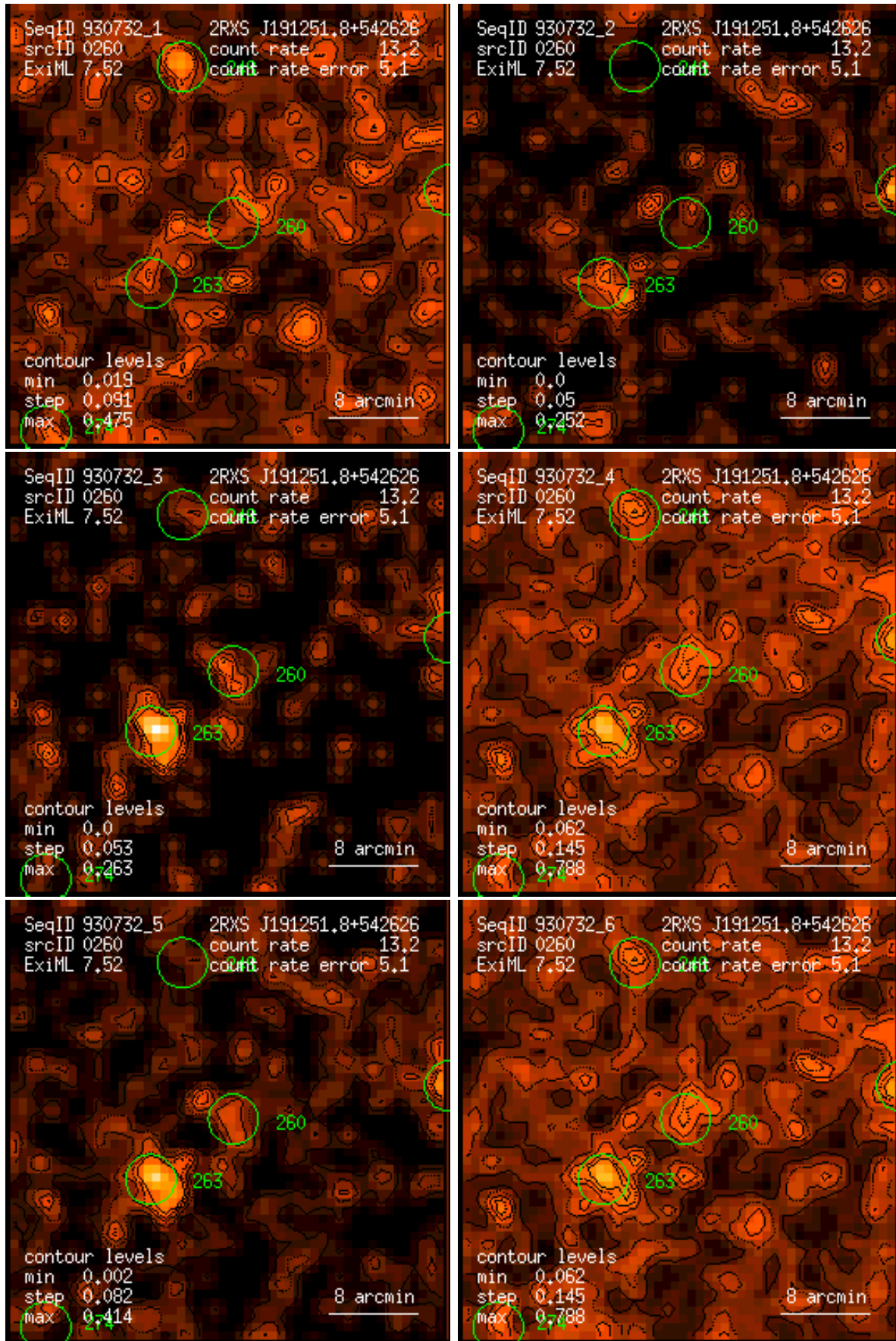
Figure 260: RASS 930732: detection 0260: band rate images, Gaussian filter: (1) PSPC channels 11 – 41, (2) 52 – 90, (3) 91 – 201, (4) 11 – 235, (5) 52 – 201, (6) 11 – 201. Broad band rates in counts/ks. Band rate contour levels in counts/ks/arcmin 2 .
