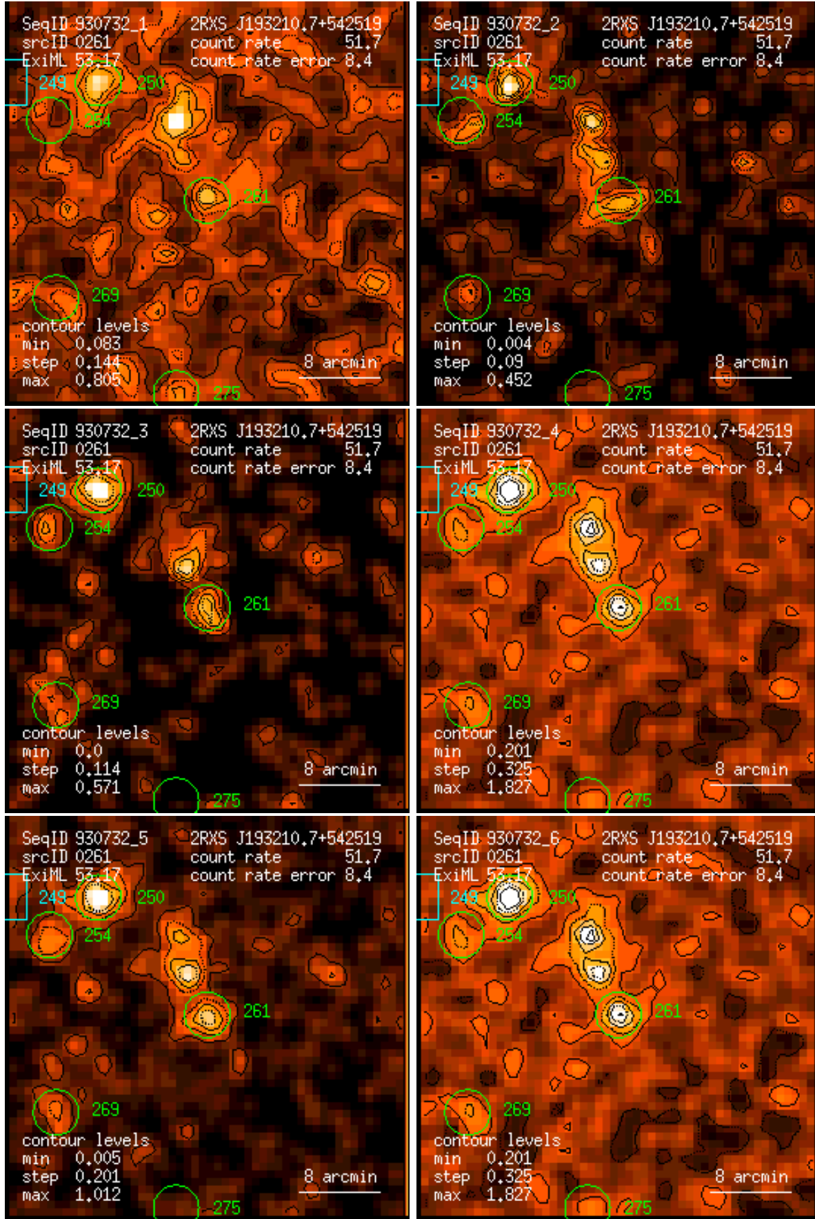
Figure 261: RASS 930732: detection 0261: band rate images, Gaussian filter: (1) PSPC channels 11 – 41, (2) 52 – 90, (3) 91 – 201, (4) 11 – 235, (5) 52 – 201, (6) 11 – 201. Broad band rates in counts/ks. Band rate contour levels in counts/ks/arcmin 2 .
