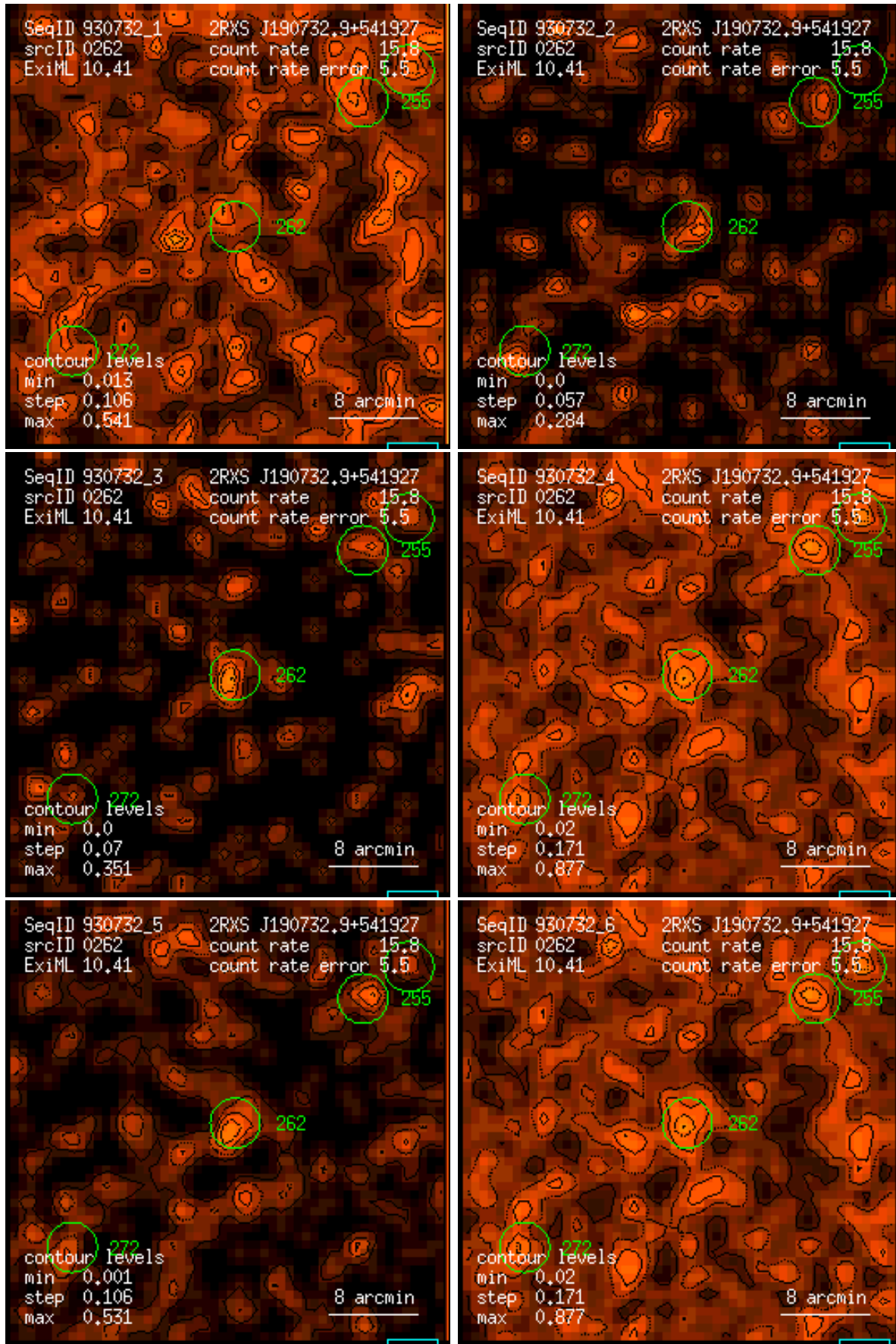
Figure 262: RASS 930732: detection 0262: band rate images, Gaussian filter: (1) PSPC channels 11 – 41, (2) 52 – 90, (3) 91 – 201, (4) 11 – 235, (5) 52 – 201, (6) 11 – 201. Broad band rates in counts/ks. Band rate contour levels in counts/ks/arcmin 2 .
