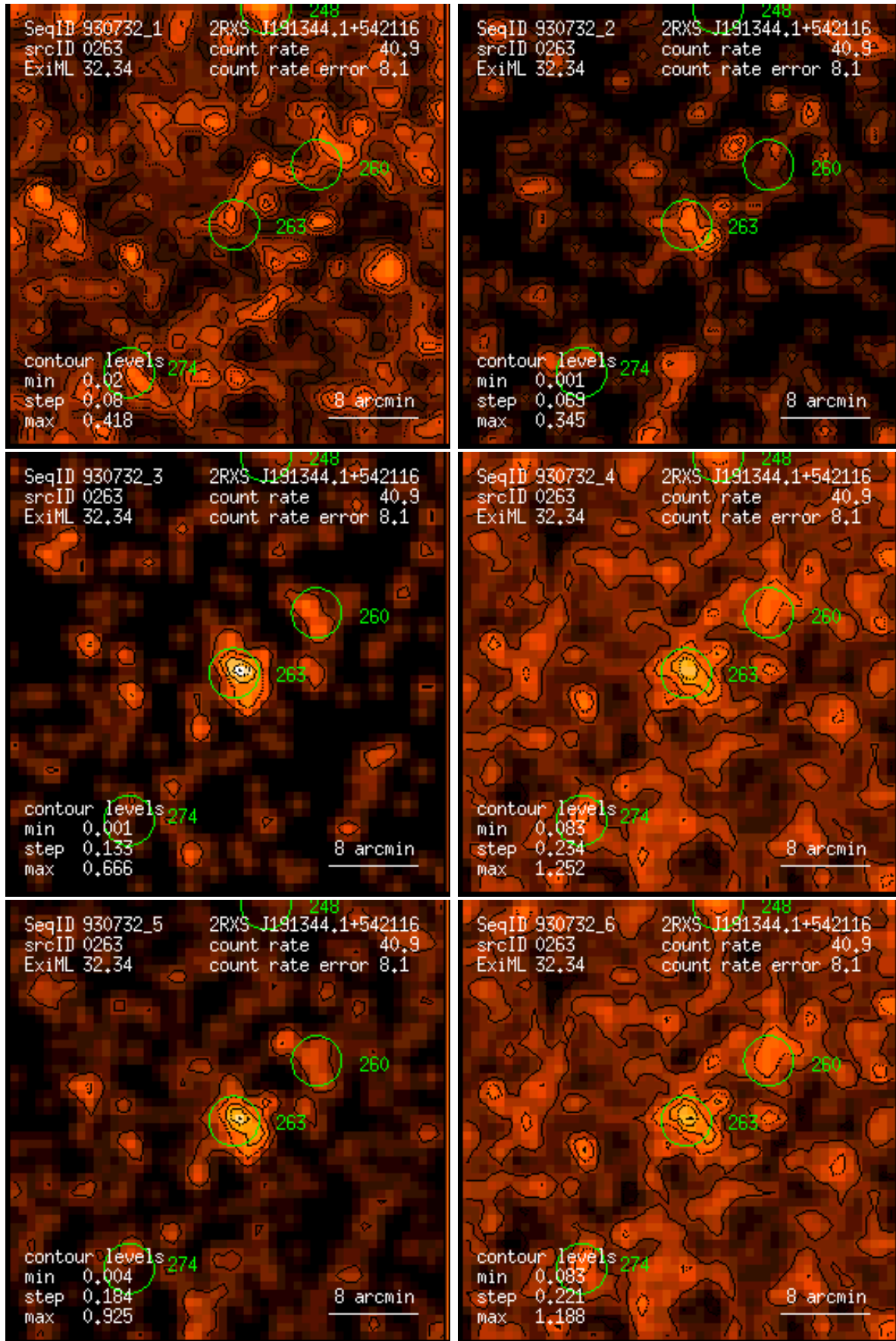
Figure 263: RASS 930732: detection 0263: band rate images, Gaussian filter: (1) PSPC channels 11 – 41, (2) 52 – 90, (3) 91 – 201, (4) 11 – 235, (5) 52 – 201, (6) 11 – 201. Broad band rates in counts/ks. Band rate contour levels in counts/ks/arcmin 2 .
