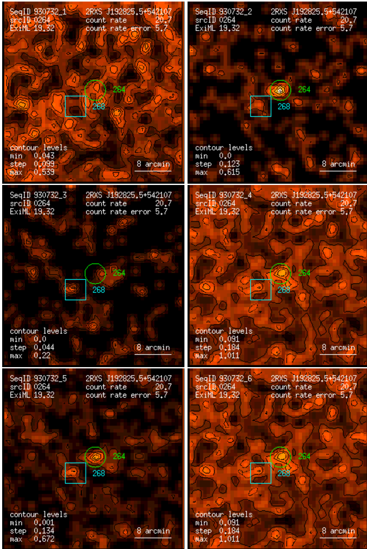
Figure 264: RASS 930732: detection 0264: band rate images, Gaussian filter: (1) PSPC channels 11 – 41, (2) 52 – 90, (3) 91 – 201, (4) 11 – 235, (5) 52 – 201, (6) 11 – 201. Broad band rates in counts/ks. Band rate contour levels in counts/ks/arcmin 2 .
