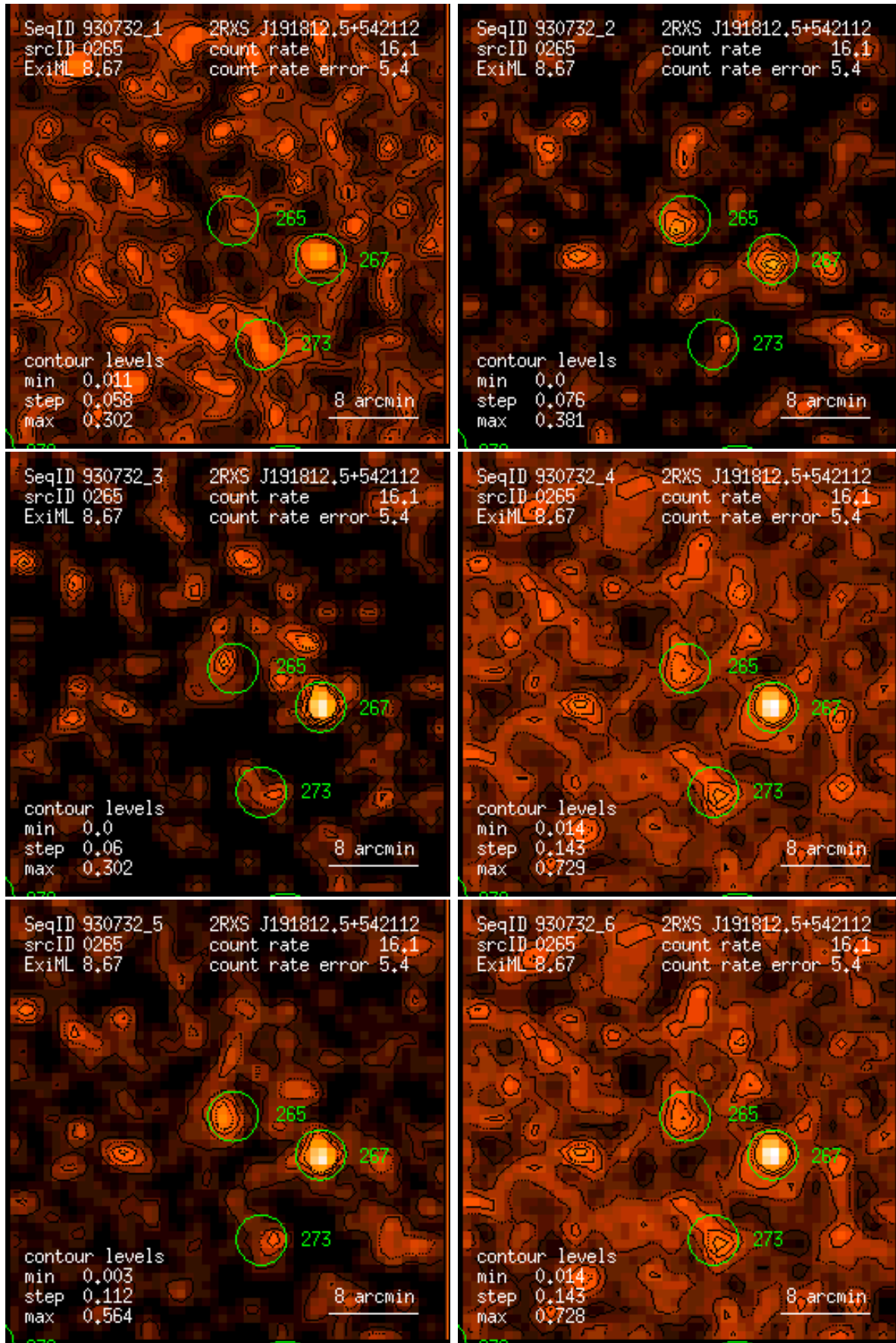
Figure 265: RASS 930732: detection 0265: band rate images, Gaussian filter: (1) PSPC channels 11 – 41, (2) 52 – 90, (3) 91 – 201, (4) 11 – 235, (5) 52 – 201, (6) 11 – 201. Broad band rates in counts/ks. Band rate contour levels in counts/ks/arcmin 2 .
