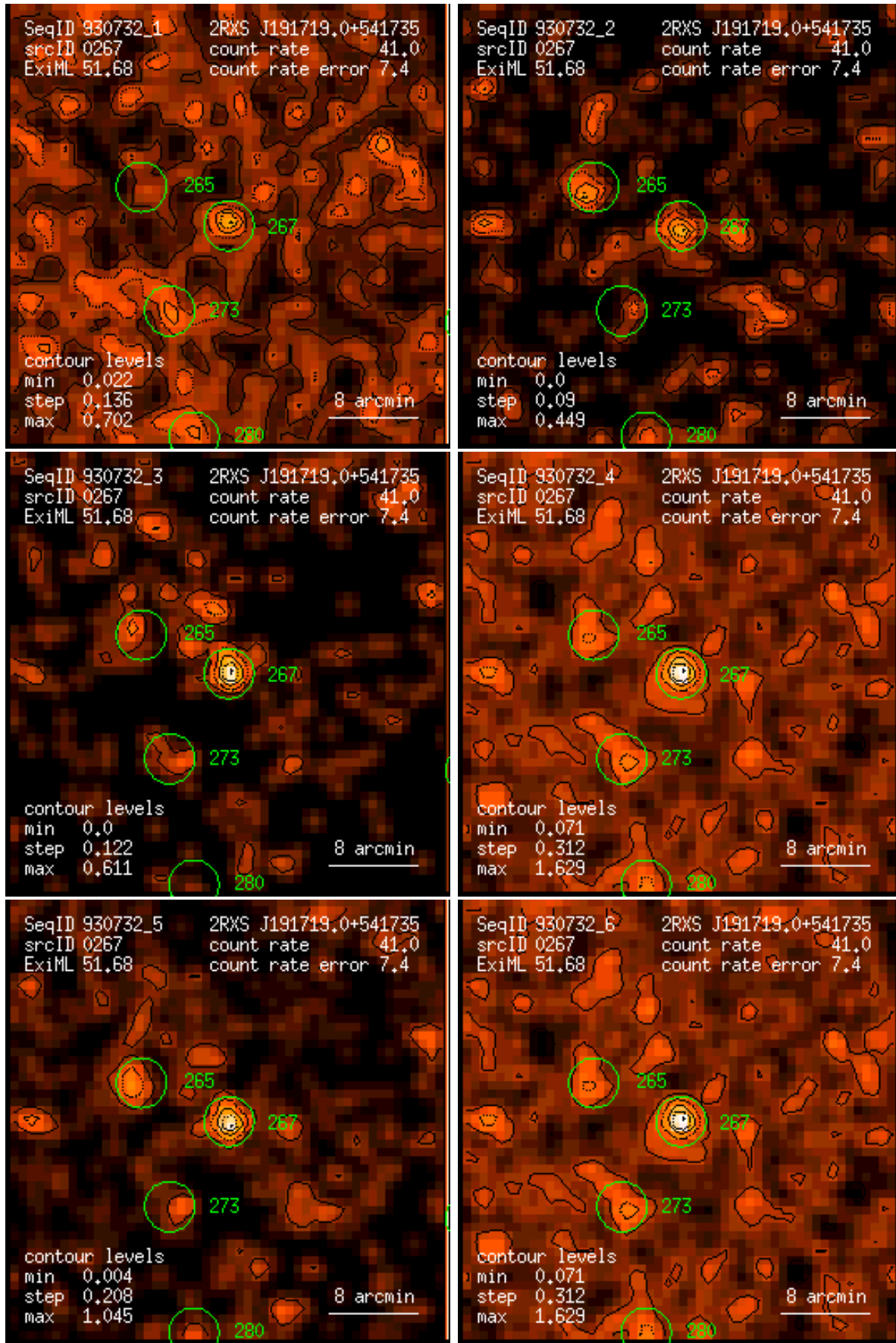
Figure 267: RASS 930732: detection 0267: band rate images, Gaussian filter: (1) PSPC channels 11 – 41, (2) 52 – 90, (3) 91 – 201, (4) 11 – 235, (5) 52 – 201, (6) 11 – 201. Broad band rates in counts/ks. Band rate contour levels in counts/ks/arcmin 2 .
