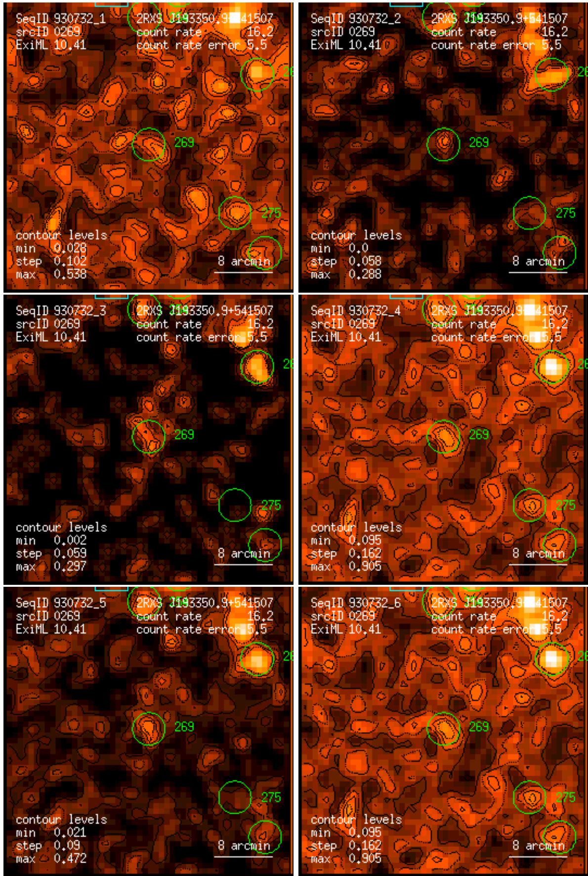
Figure 269: RASS 930732: detection 0269: band rate images, Gaussian filter: (1) PSPC channels 11 – 41, (2) 52 – 90, (3) 91 – 201, (4) 11 – 235, (5) 52 – 201, (6) 11 – 201. Broad band rates in counts/ks. Band rate contour levels in counts/ks/arcmin 2 .
