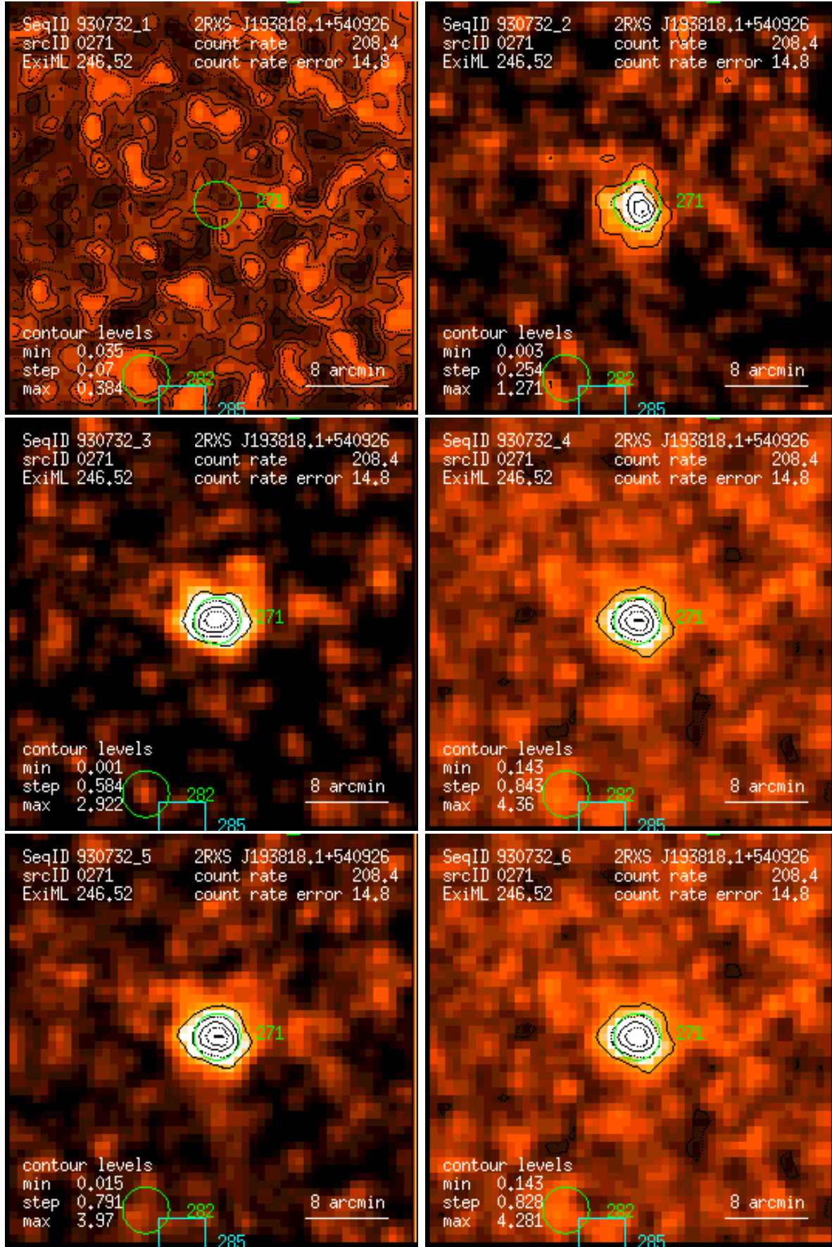
Figure 271: RASS 930732: detection 0271: band rate images, Gaussian filter: (1) PSPC channels 11 – 41, (2) 52 – 90, (3) 91 – 201, (4) 11 – 235, (5) 52 – 201, (6) 11 – 201. Broad band rates in counts/ks. Band rate contour levels in counts/ks/arcmin 2 .
