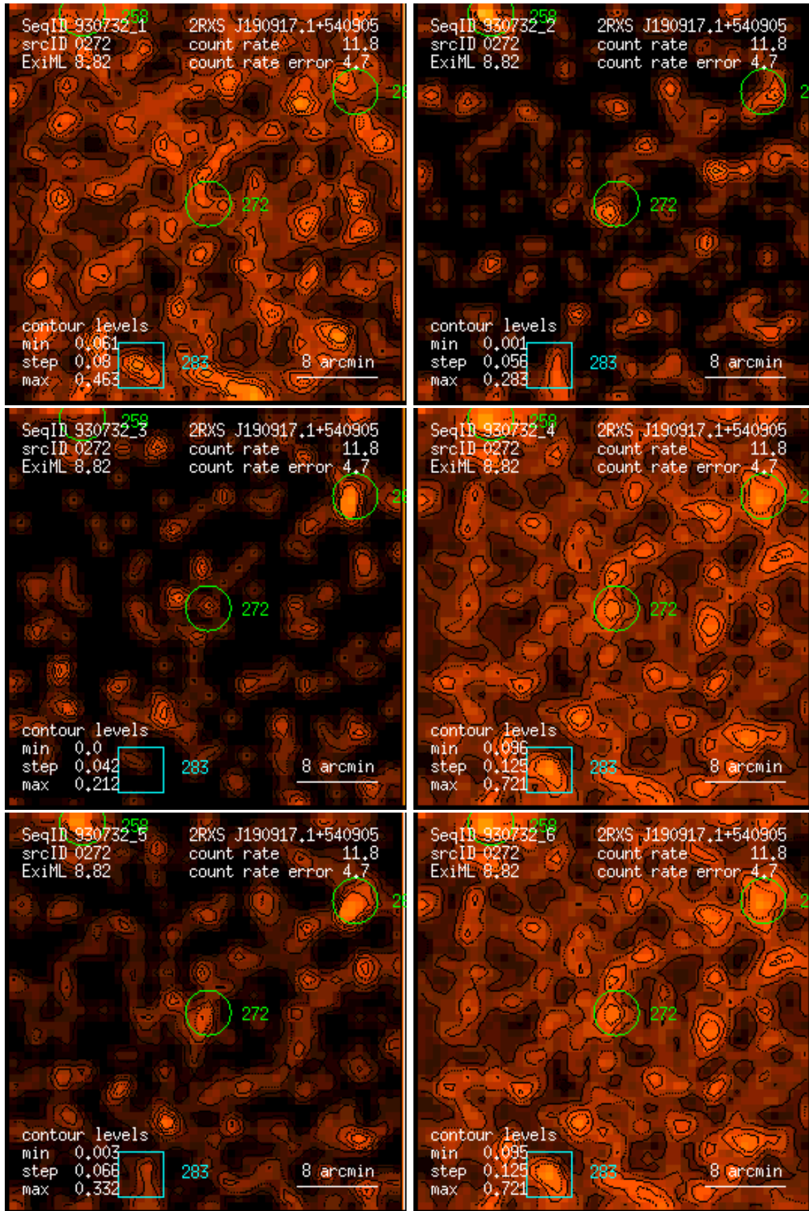
Figure 272: RASS 930732: detection 0272: band rate images, Gaussian filter: (1) PSPC channels 11 – 41, (2) 52 – 90, (3) 91 – 201, (4) 11 – 235, (5) 52 – 201, (6) 11 – 201. Broad band rates in counts/ks. Band rate contour levels in counts/ks/arcmin 2 .
