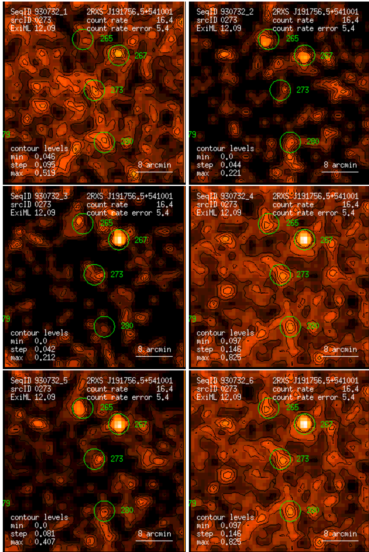
Figure 273: RASS 930732: detection 0273: band rate images, Gaussian filter: (1) PSPC channels 11 – 41, (2) 52 – 90, (3) 91 – 201, (4) 11 – 235, (5) 52 – 201, (6) 11 – 201. Broad band rates in counts/ks. Band rate contour levels in counts/ks/arcmin 2 .
