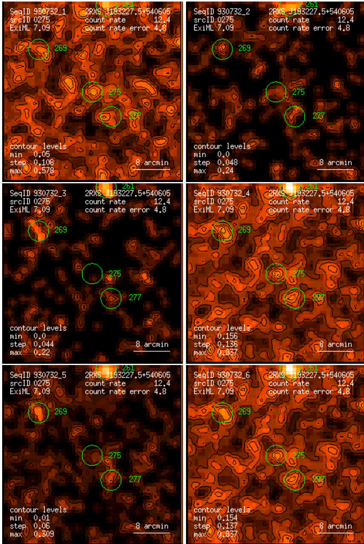
Figure 275: RASS 930732: detection 0275: band rate images, Gaussian filter: (1) PSPC channels 11 – 41, (2) 52 – 90, (3) 91 – 201, (4) 11 – 235, (5) 52 – 201, (6) 11 – 201. Broad band rates in counts/ks. Band rate contour levels in counts/ks/arcmin 2 .
