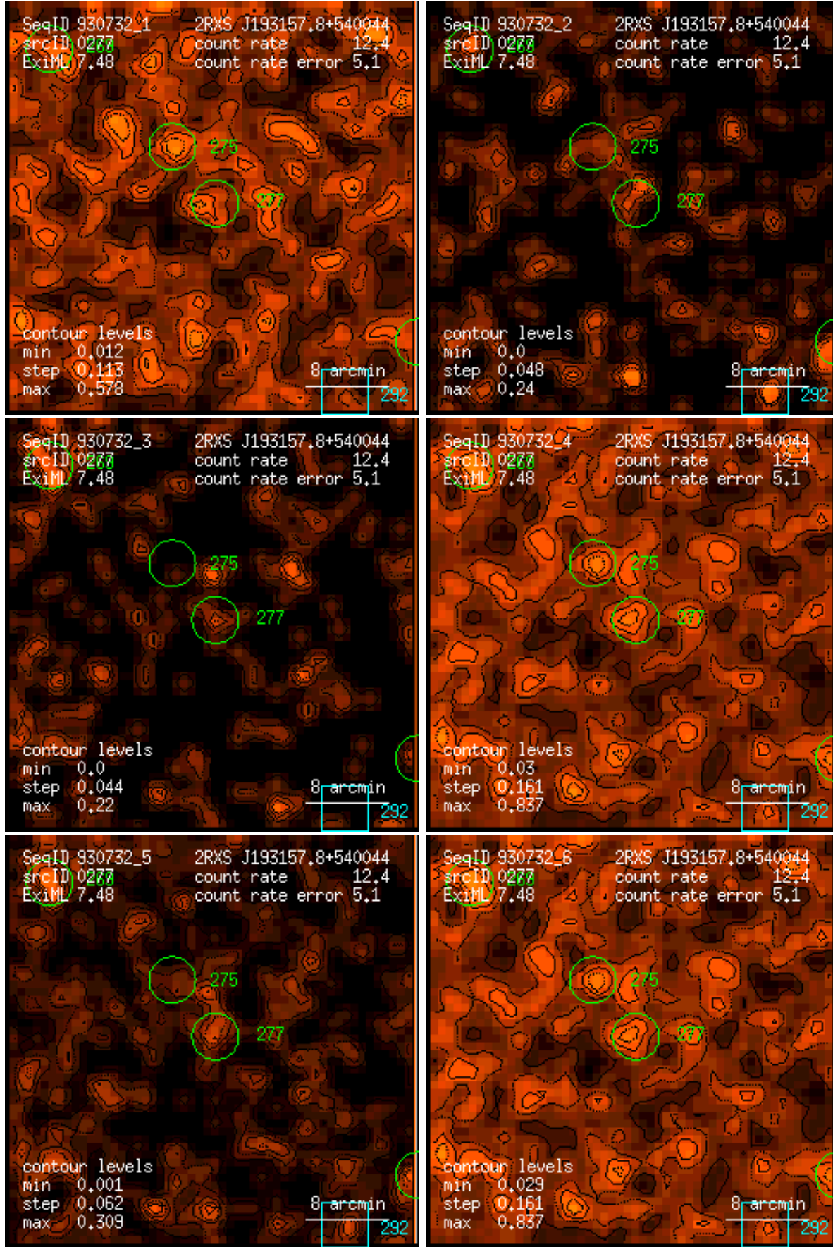
Figure 277: RASS 930732: detection 0277: band rate images, Gaussian filter: (1) PSPC channels 11 – 41, (2) 52 – 90, (3) 91 – 201, (4) 11 – 235, (5) 52 – 201, (6) 11 – 201. Broad band rates in counts/ks. Band rate contour levels in counts/ks/arcmin 2 .
