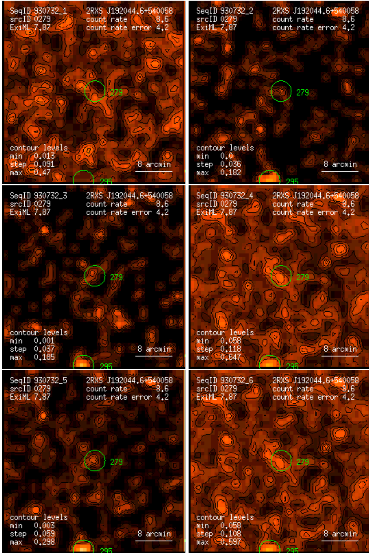
Figure 279: RASS 930732: detection 0279: band rate images, Gaussian filter: (1) PSPC channels 11 – 41, (2) 52 – 90, (3) 91 – 201, (4) 11 – 235, (5) 52 – 201, (6) 11 – 201. Broad band rates in counts/ks. Band rate contour levels in counts/ks/arcmin 2 .
