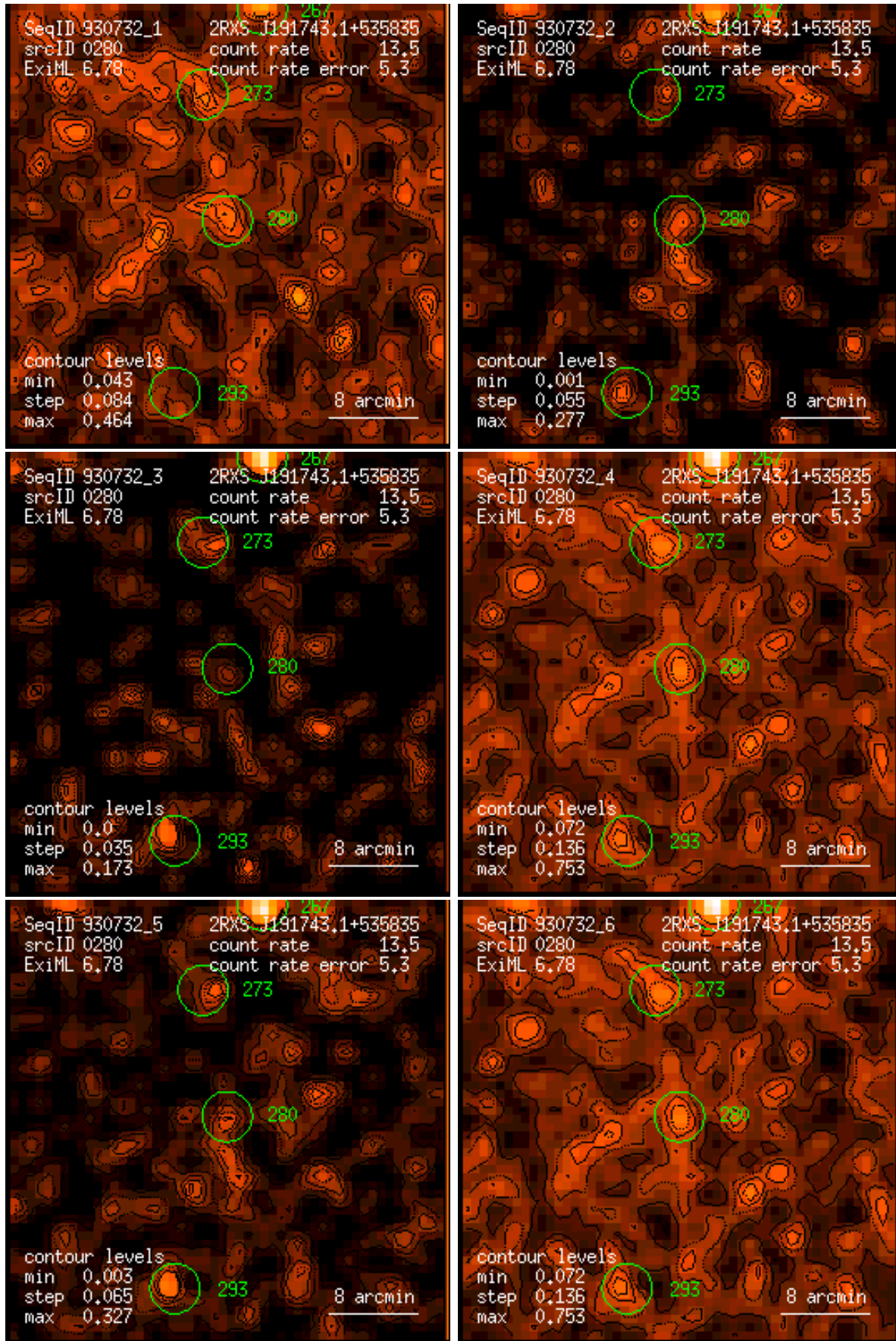
Figure 280: RASS 930732: detection 0280: band rate images, Gaussian filter: (1) PSPC channels 11 – 41, (2) 52 – 90, (3) 91 – 201, (4) 11 – 235, (5) 52 – 201, (6) 11 – 201. Broad band rates in counts/ks. Band rate contour levels in counts/ks/arcmin 2 .
