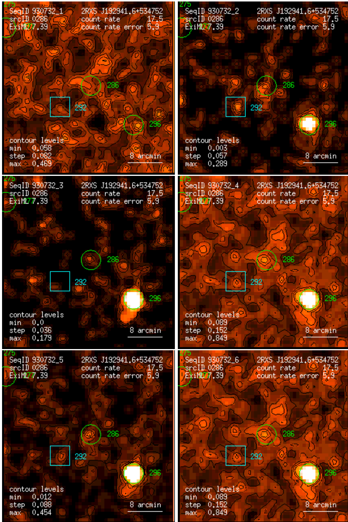
Figure 286: RASS 930732: detection 0286: band rate images, Gaussian filter: (1) PSPC channels 11 – 41, (2) 52 – 90, (3) 91 – 201, (4) 11 – 235, (5) 52 – 201, (6) 11 – 201. Broad band rates in counts/ks. Band rate contour levels in counts/ks/arcmin 2 .
